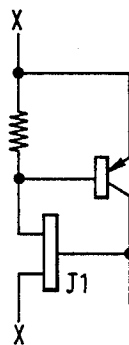
FIG. 4. (PRIOR ART)
