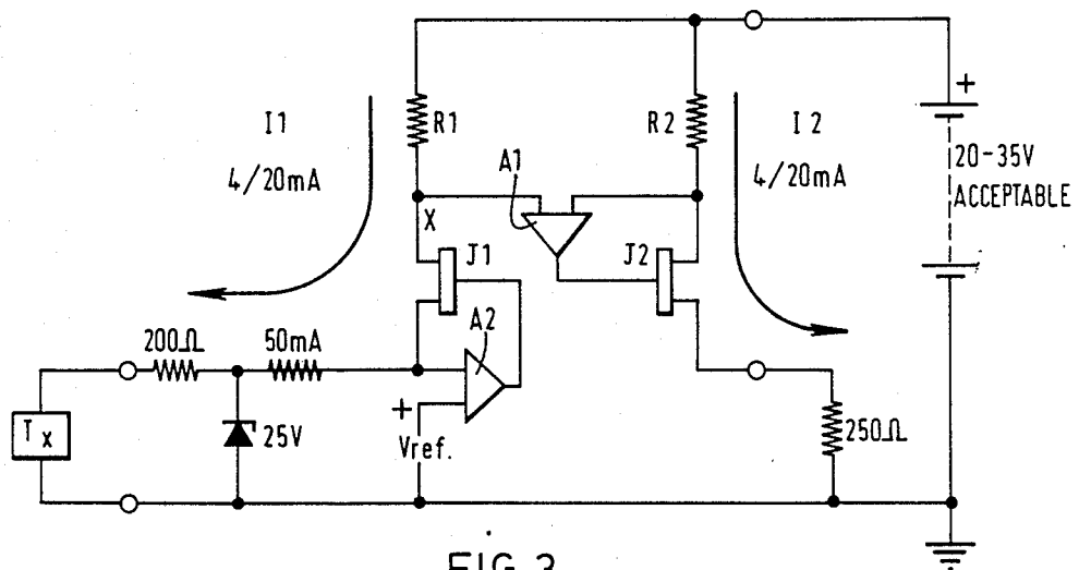
FIG. 3. (PRIOR ART)
