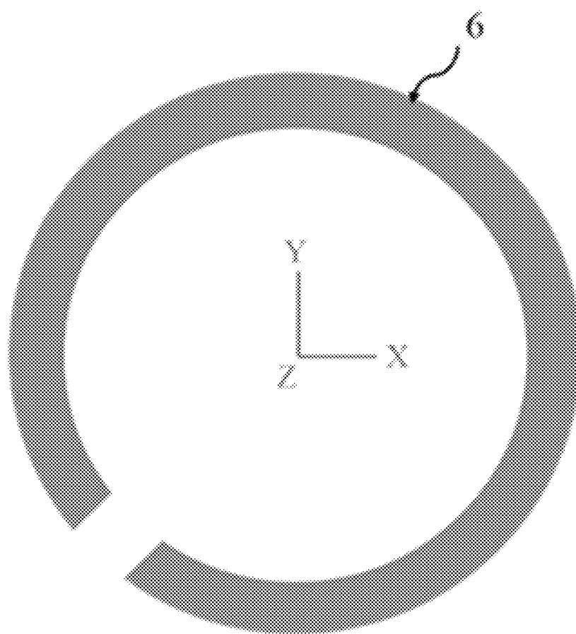
FIG. 3 (b) Element in a dipole structure
