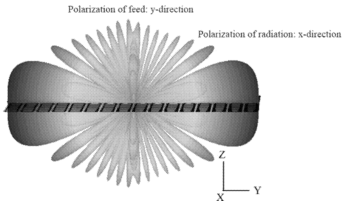
FIG. 7 (b) Space waves illuminated positively (Array of dipoles)
