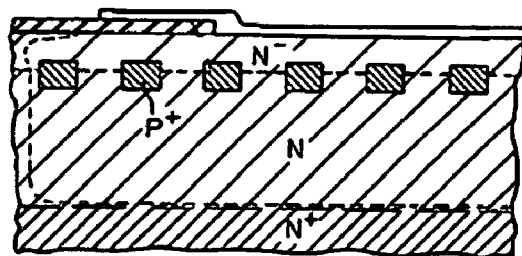
Fig. 1C (Prior Art)
