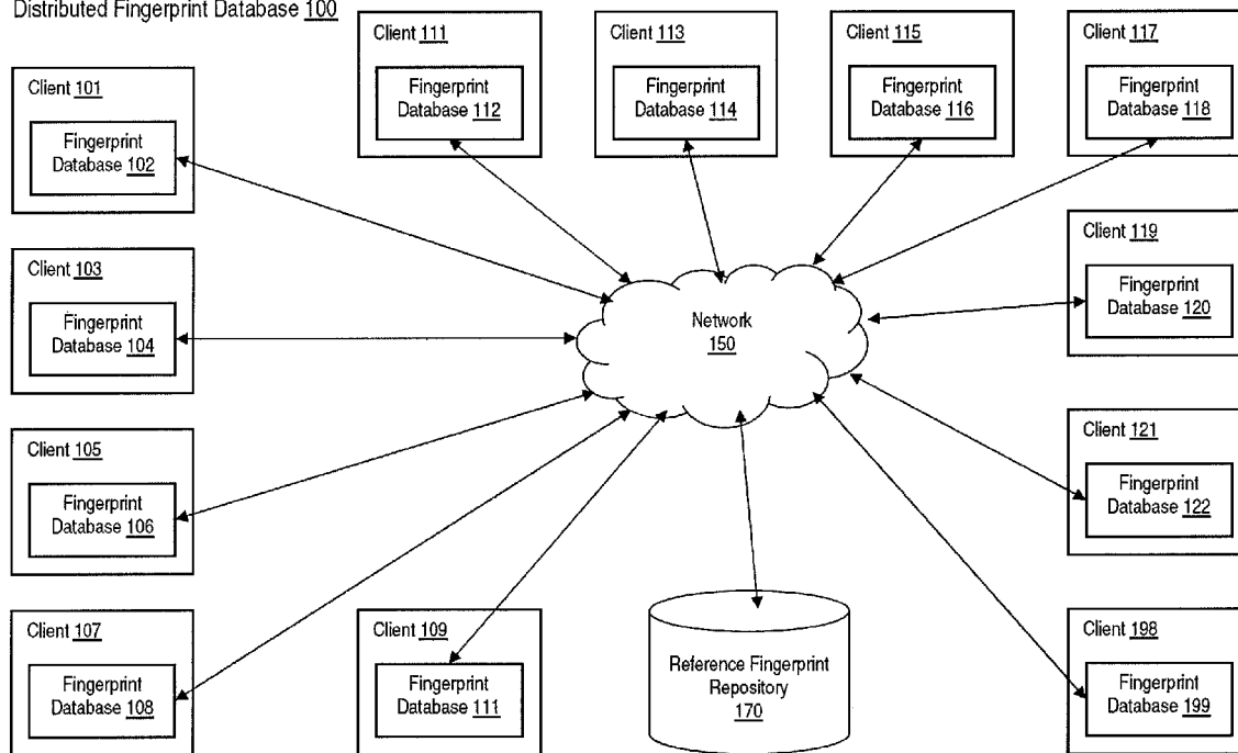
Distributed Fingerprint Database 100
