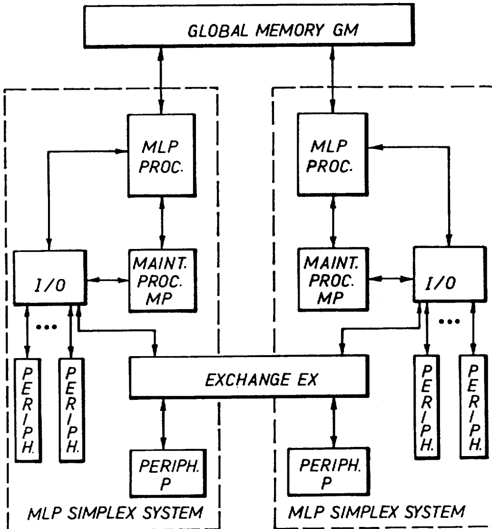
FIG. 1 OVERALL SYSTEM
