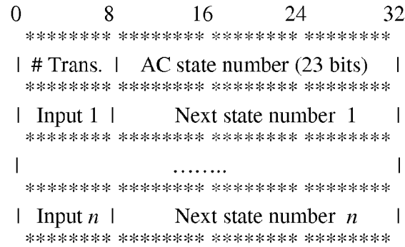
Suffix Tree Data Structure
