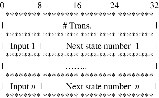
DAWG Data Structure
