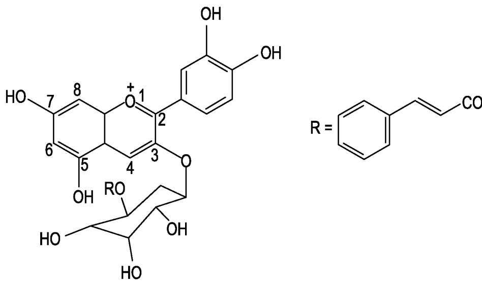
II: CYANIDIN -3- GLUCOSIDE-COUMARATE
