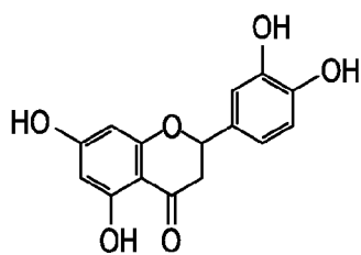
ERIODICTYOL
