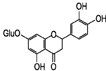
ERIODICTYOL-7-GLUCOSIDE
