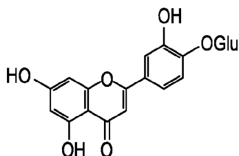
LUTEOLIN-4'-GLUCOSIDE
