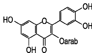
QUERCETIN-3-ARABINOSIDE
