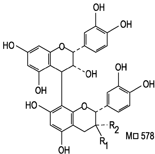
1. CATECHIN
