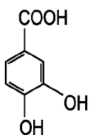
PROTOCATECHUIC ACID
