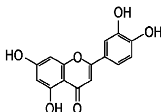
LUTEOLIN
