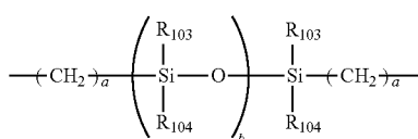
Chemical structure I-b
