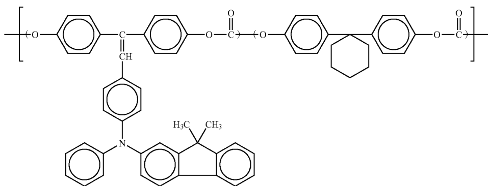
Specific compound chemical structure 14
