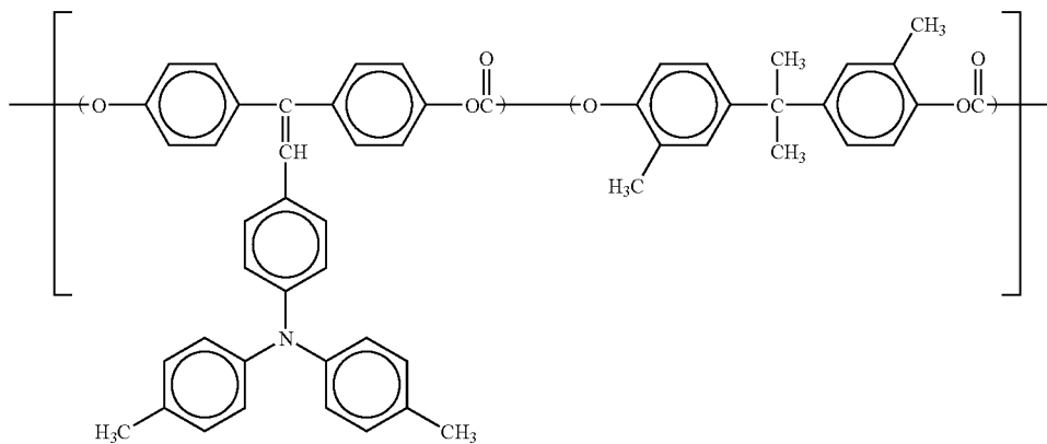
Specific compound chemical structure 12
