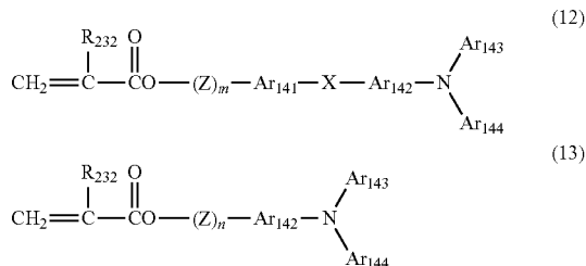
Chemical structures 12 and 13
