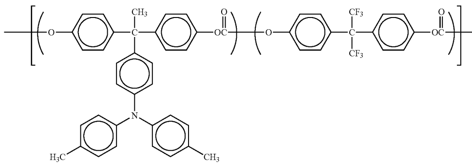
Specific compound chemical structure 2
