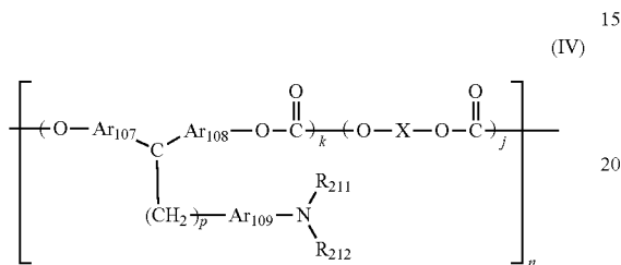
Chemical structure VI
