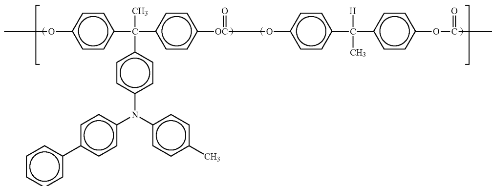
Specific compound chemical structure 4
