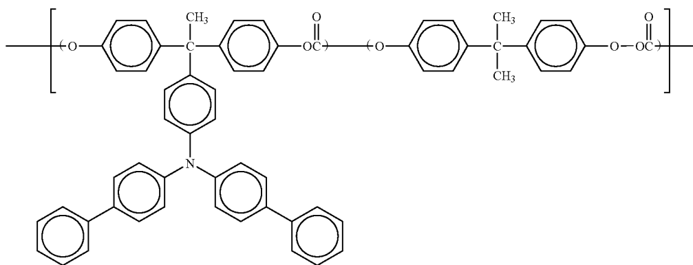
Specific compound chemical structure 2
