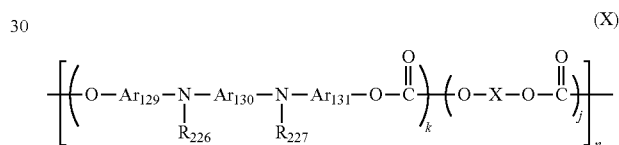
Chemical structure X
