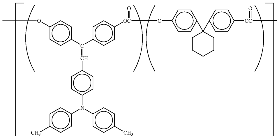
Specific compound chemical structure 11
