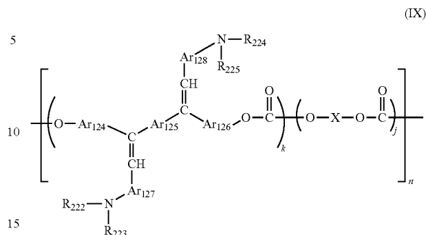
Chemical structure IX
