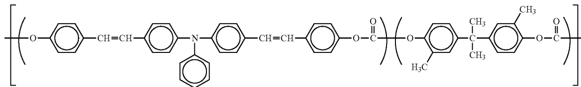
Specific compound chemical structure 26
