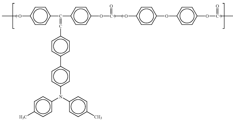
Specific compound chemical structure 13
