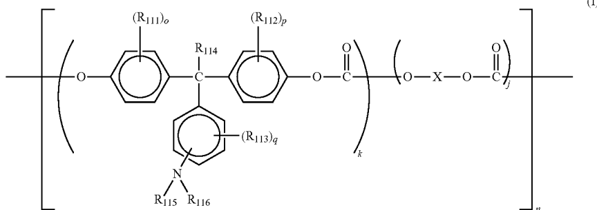
Chemical structure (I)
