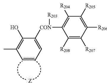
Chemical structure 10a
