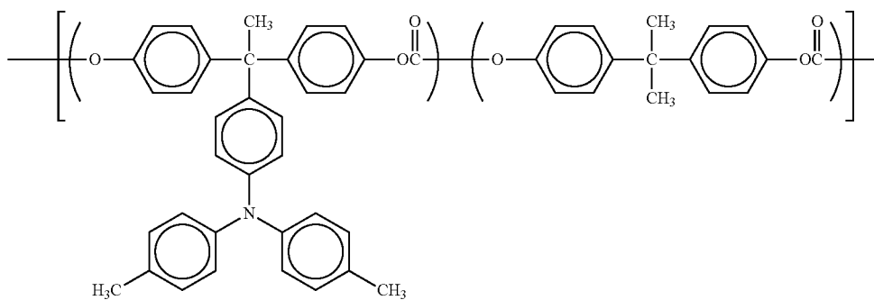
Specific compound chemical structure 5
