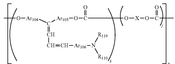
Chemical structure III
