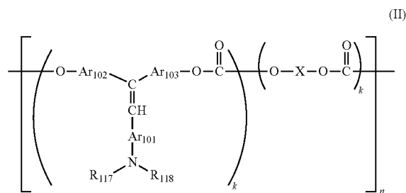
Chemical structure II
