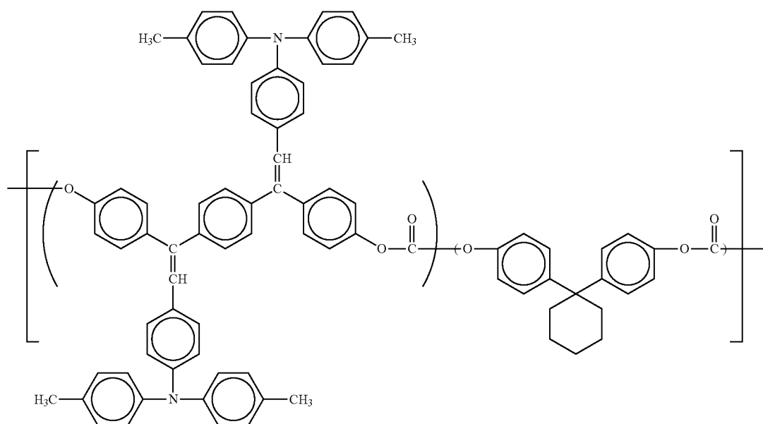
Specific compound chemical structure 27
