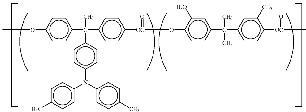
Specific compound chemical structure 9
