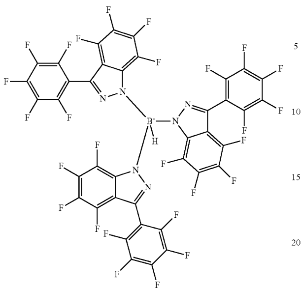
Chemical Formula: C_{39}HBF_{27}LiN_6 Molecular Weight: 1084.19
