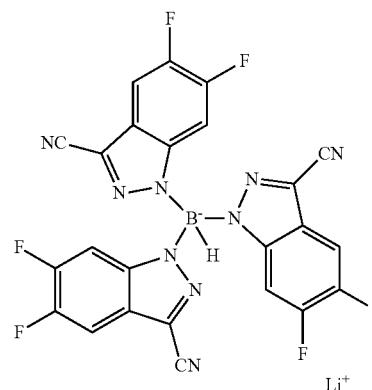
Chemical Formula: C_{24}H_7BF_6LiN_9 Molecular Weight: 553.12
