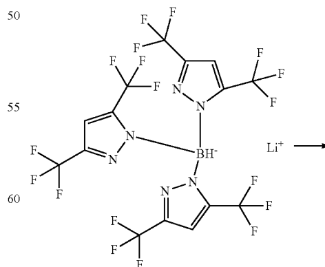
Chemical Formula: C_{15}H_4BF_{18}LiN_6 Molecular Weight: 627.96
