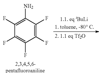
Scheme 1: Synthesis of bis((1,1,1-trifluoro-N-(perfluorophenyl)methyl)-sulfonamido)zinc
