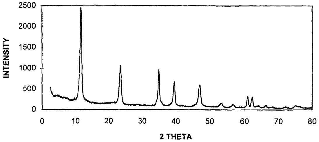
FIGURE 1: X-RAY DIFFRACTION PATTERN FOR COMMERCIAL ANIONIC CLAY
