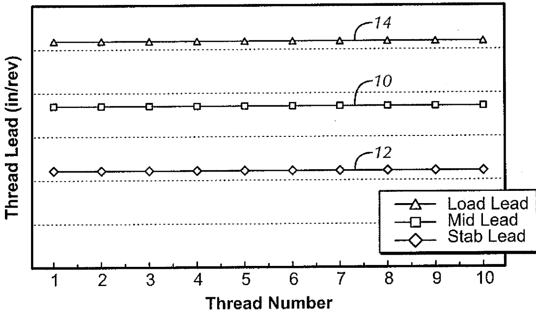
FIG. 3 (Prior Art)
