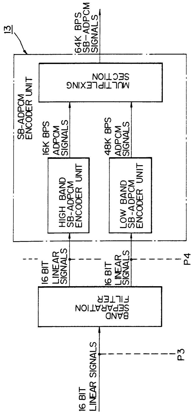
Fig. 4 (PRIOR ART)
