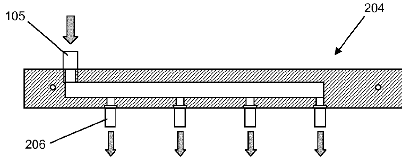
Figure 3 Sectional view in XZ of cleaning fluid manifold
