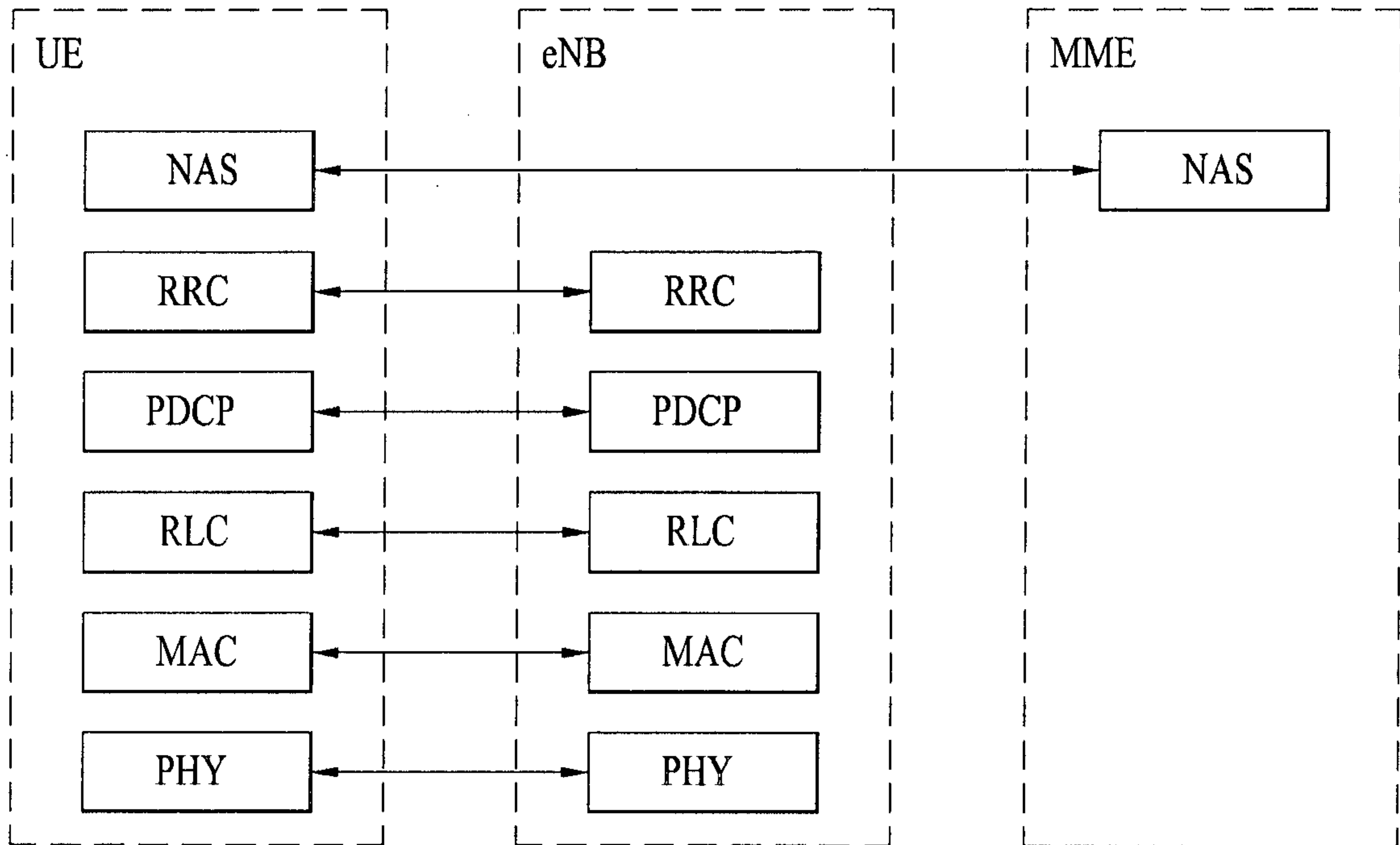
(A) CONTROL-PLANE PROTOCOL STACK
