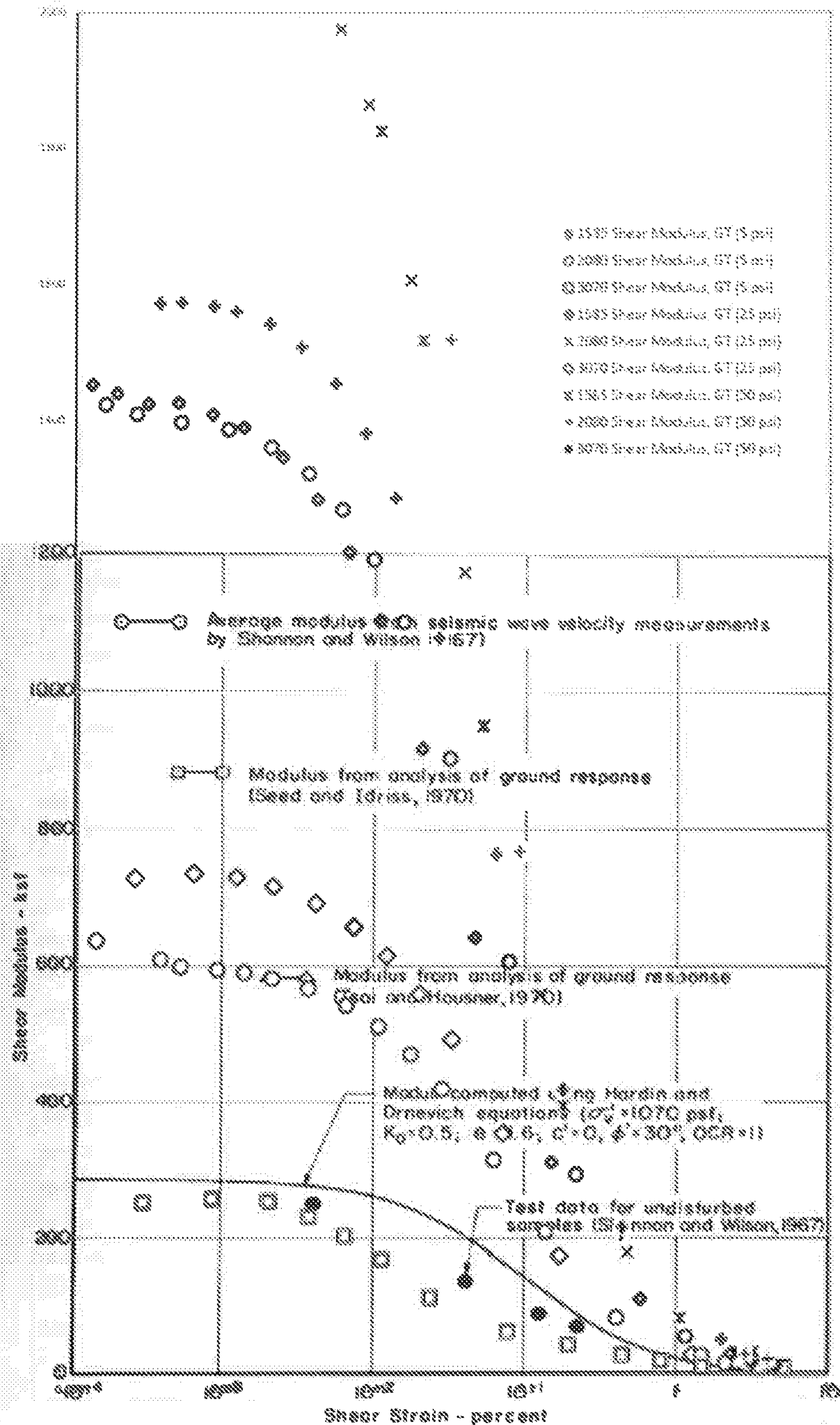
Fig. 6 Comparison of Shear Modulus against Clay Soil
