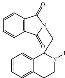
3-Oxomethylene-2-(1,2,3,4-tetrahydro-isoquinolin-1-ylmethyl)-2,3-dihydro-isoindol-1-one
