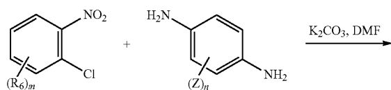
Scheme II
