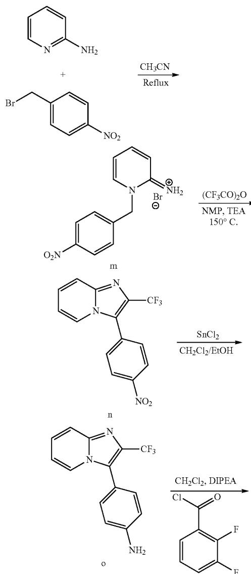
Scheme VIII
