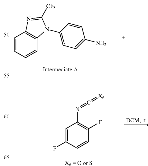
Scheme IV
