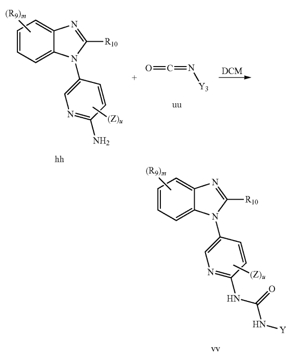
Scheme XVII
