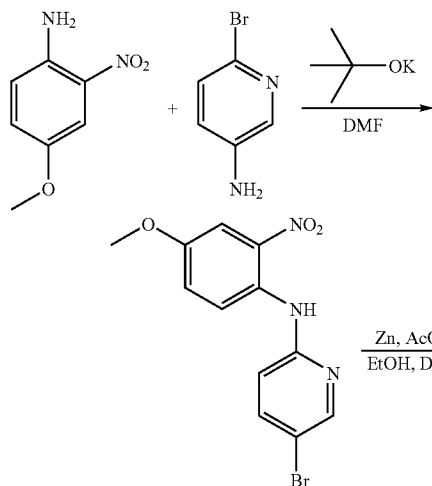
Scheme XII
