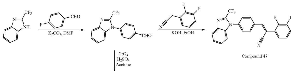
Scheme VII
