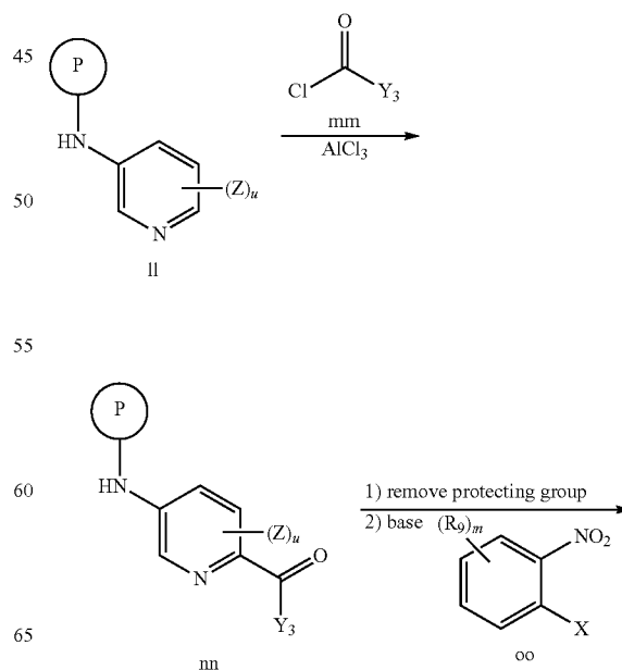
Scheme XV
