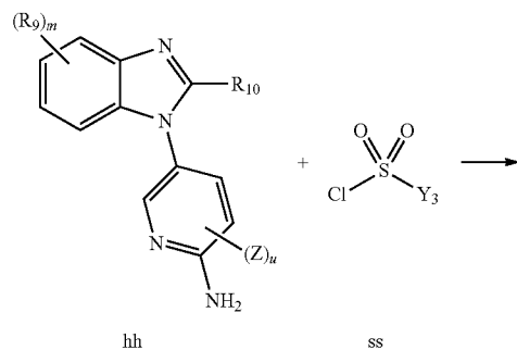
Scheme XVI
