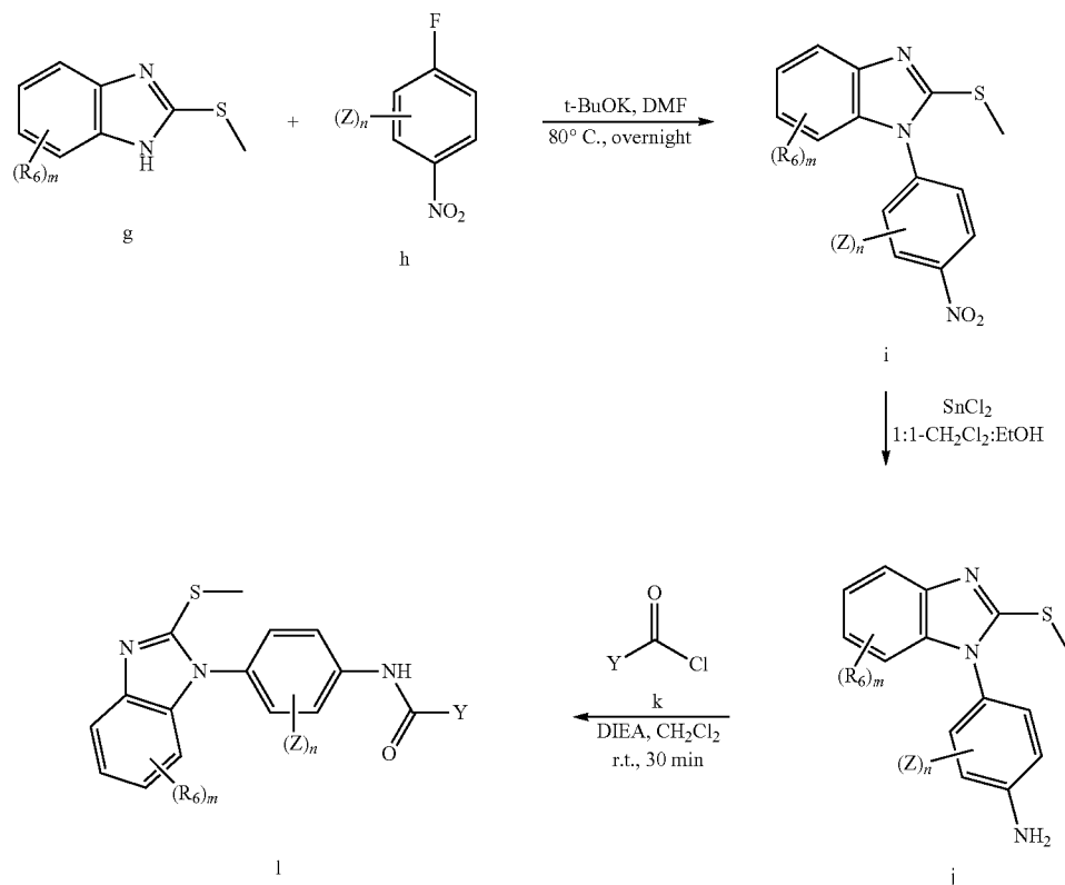
Scheme III
