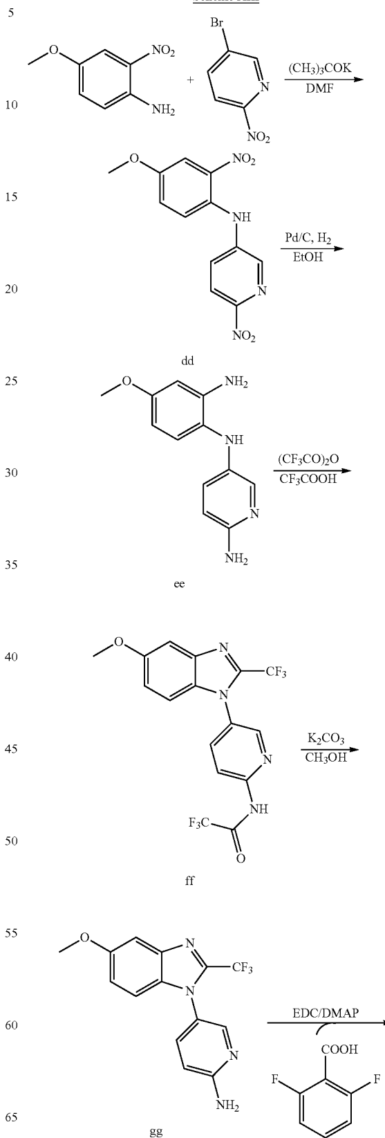
Scheme XIII
