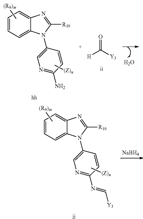
Scheme XIV
