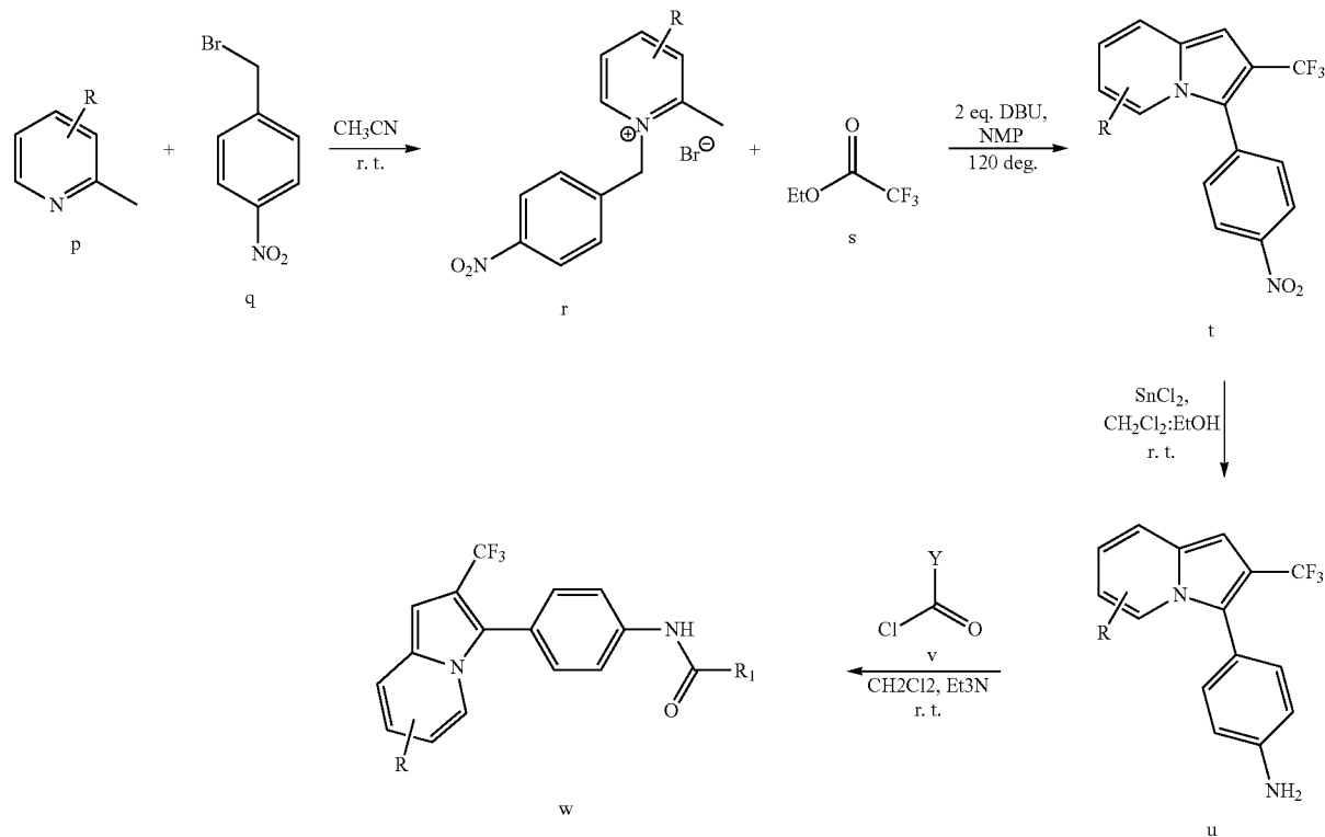
Scheme IX
