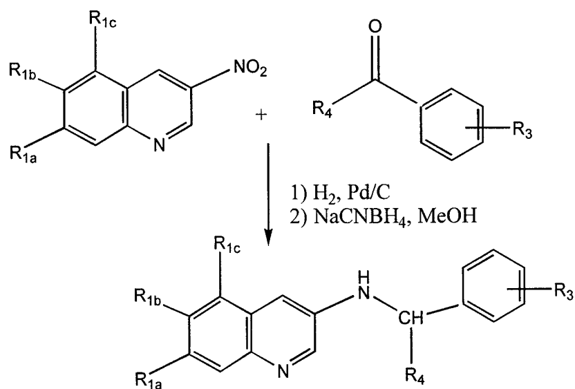
Scheme III
