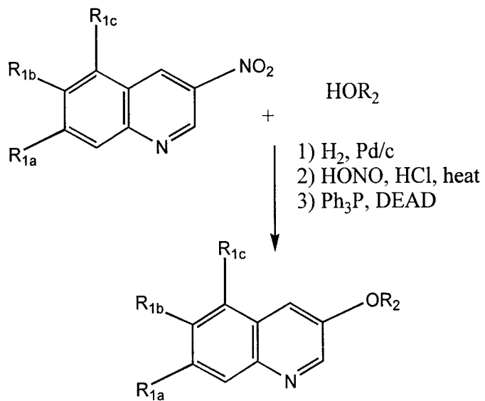
Scheme V
