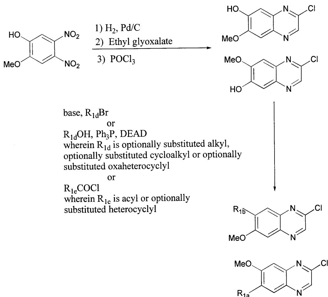
Scheme VII
