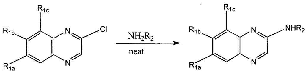
Scheme II
