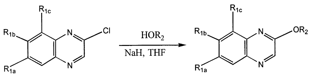
Scheme III
