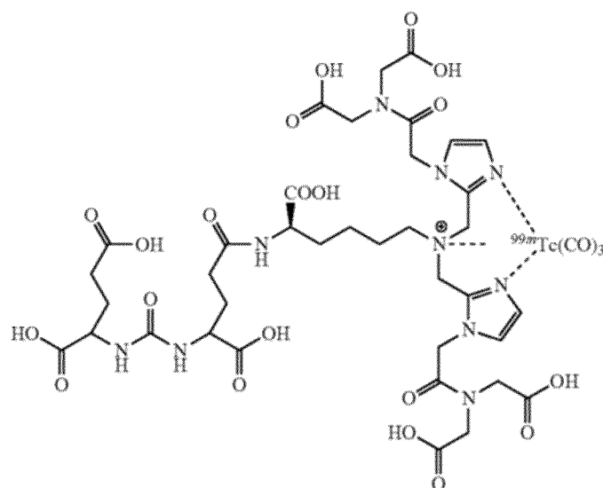
^{99m}\text{Tc} -MIP-1404,
