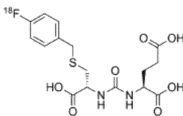
[18F]DCFBC,
