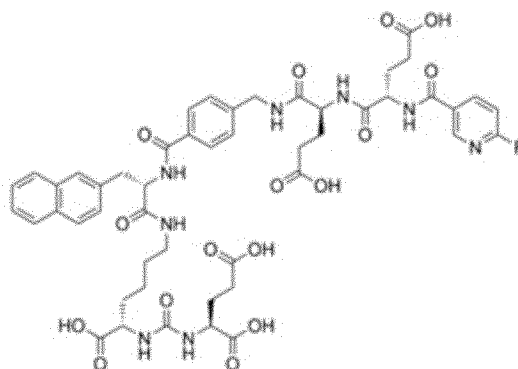
PSMA-1007,
