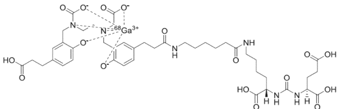
68 Ga-PSMA-HBED-CC,
