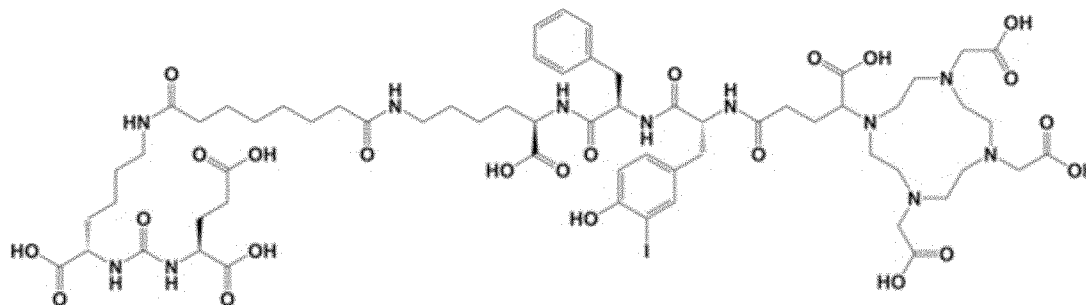
PSMA-I&amp;T,
