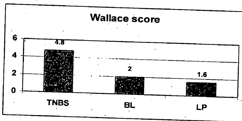
Figure 6: Wallace scores
