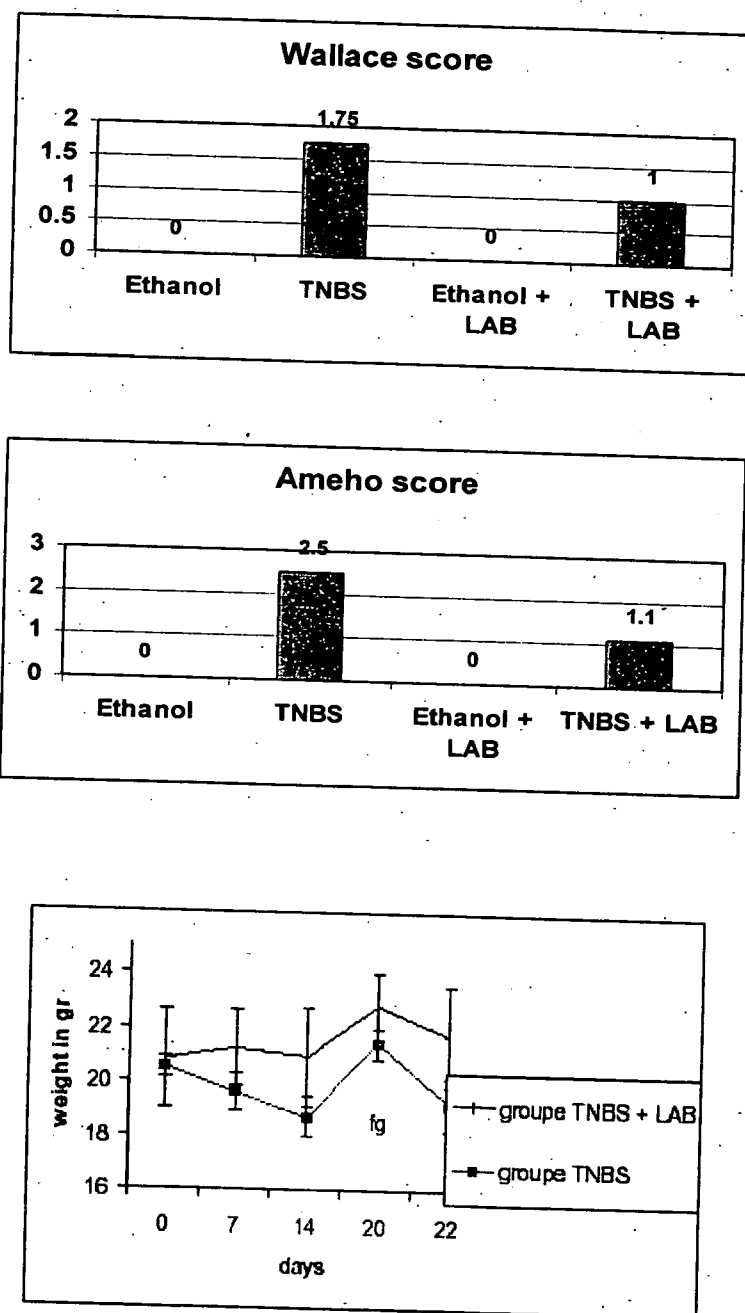
Figure 2: Wallace and Ameho scores, and weight evolution
