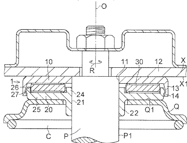
FIG. 15 (PRIOR ART)
