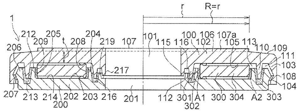
FIG. 14 (PRIOR ART)
