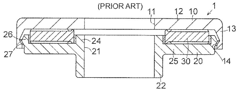
FIG. 15 (PRIOR ART)
