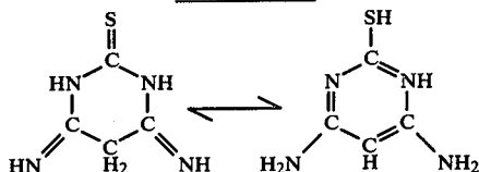
Hexahydro-4,6-diimino-1,3-pyrimidine-2-thione or 2-mercapto-4,6-diamino-1,3-pyrimidine
