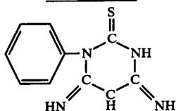
Hexahydro-1-phenyl-4,6-diimino-s-triazine-2-thione
