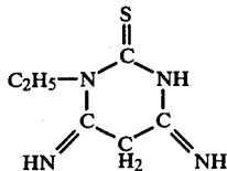
Hexahydro-1-ethyl-4,6-diimino-1,3-pyrimidine-2-thione
