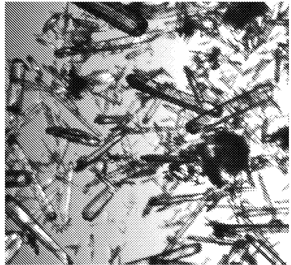
Crystal Form 3
