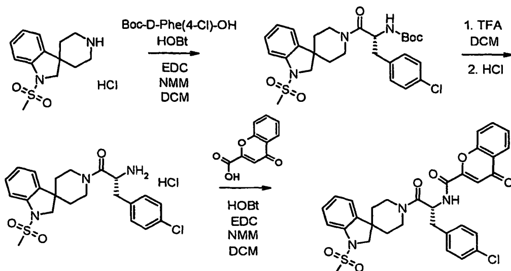
Synthesis Scheme for Example 1
