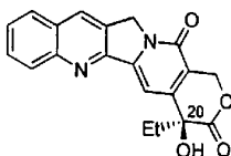
(2S)-camptothecin, CPT Rings are labeled A-E from left to right
