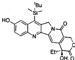
(20S)-10-Hydroxy-7-tert-butyldimethylsilylcamptothecin (DB-67)
