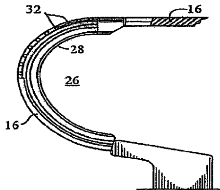
Fig. 2 PRIOR ART
