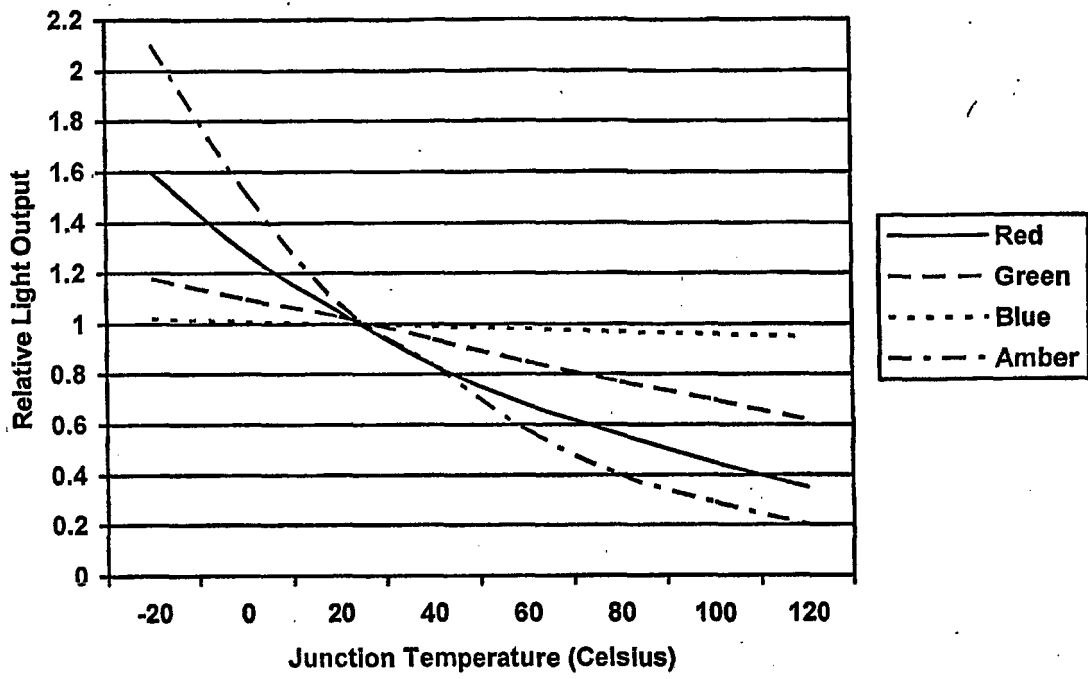
Figure 3 (Prior Art)
