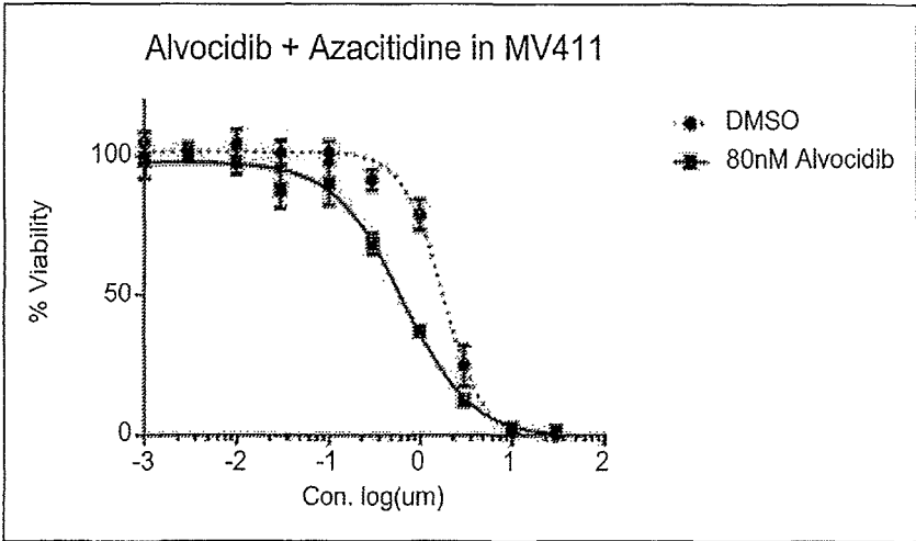
Alvocidib+Aza normalized to Alvocidib only treatment
