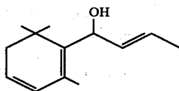
(70% trans isomer)
