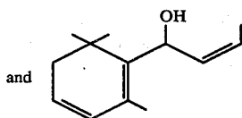
(30% cis isomer)
