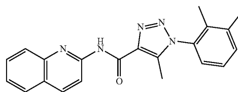
1-(2,3-Dimethylphenyl)-5-methyl-N-(quinolin-2-yl)-1H-1,2,3-triazole-4-carboxamide (42)
