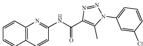
1-(3-Chlorophenyl)-5-methyl-N-(quinolin-2-yl)-1H-1,2,3-triazole-4-carboxamide (44)
