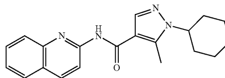
1-cyclohexyl-5-methyl-N-(quinolin-2-yl)-1H-pyrazole-4-carboxamide (142)
