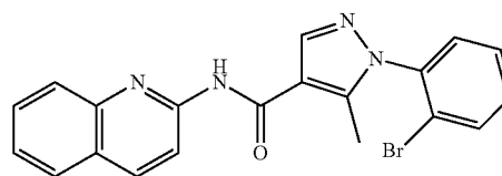
1-(2-bromophenyl)-5-methyl-N-(quinolin-2-yl)-1H-pyrazole-4-carboxamide (134)
