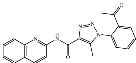
1-(2-Acetylphenyl)-5-methyl-N-(quinolin-2-yl)-1H-1,2,3-triazole-4-carboxamide (39)
