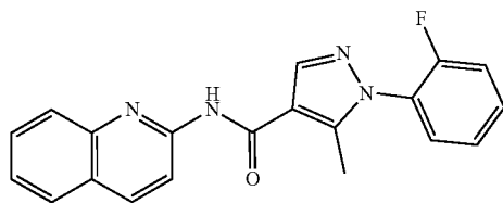
1-(2-Fluorophenyl)-5-methyl-N-(quinolin-2-yl)-1H-pyrazole-4-carboxamide (133)
