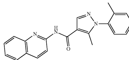
5-Methyl-N-(quinolin-2-yl)-1-(o-tolyl)-1H-pyrazole-4-carboxamide (132)
