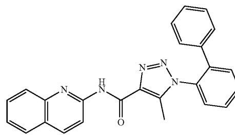
1-([1,1'-biphenyl]-2-yl)-5-methyl-N-(quinolin-2-yl)-1H-1,2,3-triazole-4-carboxamide (38)
