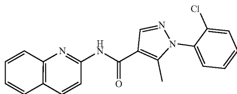
1-(2-Chlorophenyl)-5-methyl-N-(quinolin-2-yl)-1H-pyrazole-4-carboxamide (135)
