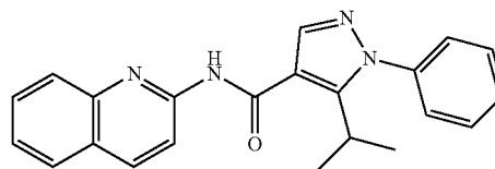
5-isopropyl-1-phenyl-N-(quinolin-2-yl)-1H-pyrazole-4-carboxamide (158)
