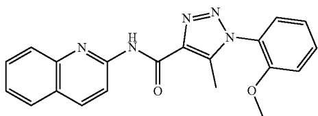
1-(2-Methoxyphenyl)-5-methyl-N-(quinolin-2-yl)-1H-1,2,3-triazole-4-carboxamide (35)
