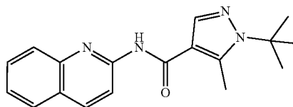
1-(Tert-butyl)-5-methyl-N-(quinolin-2-yl)-1H-pyrazole-4-carboxamide (138)
