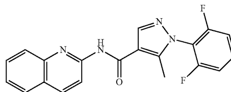
1-(2,6-difluorophenyl)-5-methyl-N-(quinolin-2-yl)-1H-pyrazole-4-carboxamide (147)
