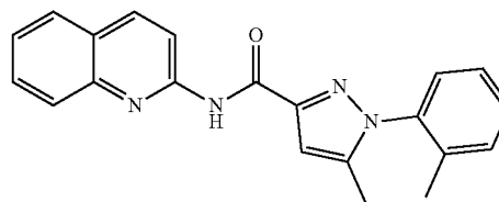
5-methyl-N-(quinolin-2-yl)-1-(o-tolyl)-1H-pyrazole-3-carboxamide (150)
