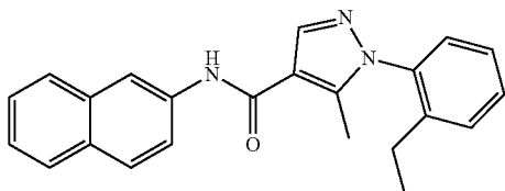
1-(2-ethylphenyl)-5-methyl-N-(naphthalen-2-yl)-1H-pyrazole-4-carboxamide (162)
