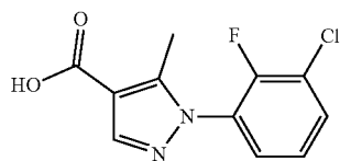
1-(3-Chloro-2-fluorophenyl)-5-methyl-1H-pyrazole-4-carboxylic acid
