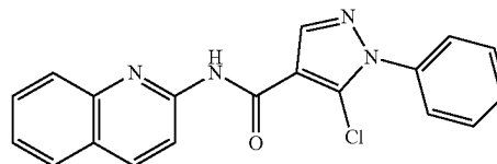
5-chloro-1-phenyl-N-(quinolin-2-yl)-1H-pyrazole-4-carboxamide (159)
