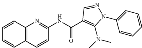
5-(dimethylamino)-1-phenyl-N-(quinolin-2-yl)-1H-pyrazole-4-carboxamide (161)
