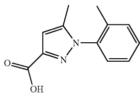
5-methyl-1-(o-tolyl)-1H-pyrazole-3-carboxylic acid
