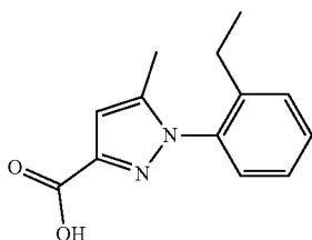
1-(2-ethylphenyl)-5-methyl-1H-pyrazole-3-carboxylic acid
