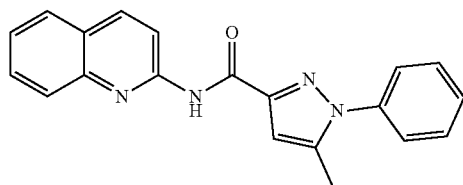
5-methyl-1-phenyl-N-(quinolin-2-yl)-1H-pyrazole-3-carboxamide (149)
