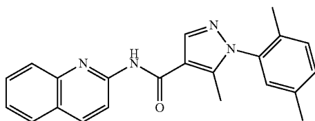
1-(2,5-dimethylphenyl)-5-methyl-N-(quinolin-2-yl)-1H-pyrazole-4-carboxamide (139)
