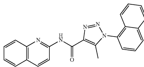
5-Methyl-1-(naphthalen-1-yl)-N-(quinolin-2-yl)-1H-1,2,3-triazole-4-carboxamide (43)
