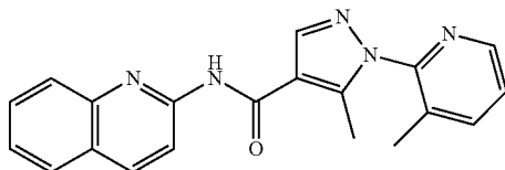
5-methyl-1-(3-methylpyridin-2-yl)-N-(quinolin-2-yl)-1H-pyrazole-4-carboxamide (145)
