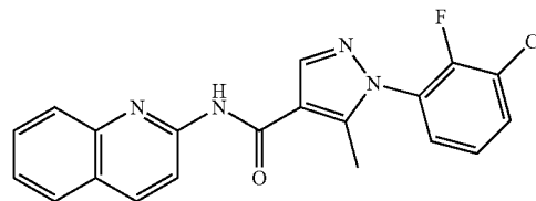
1-(3-chloro-2-fluorophenyl)-5-methyl-N-(quinolin-2-yl)-1H-pyrazole-4-carboxamide (146)
