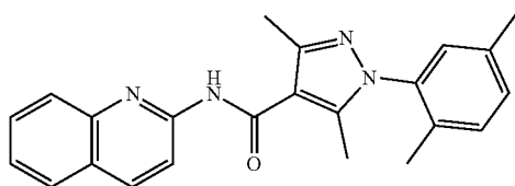
1-(2,5-dimethylphenyl)-3,5-dimethyl-N-(quinolin-2-yl)-1H-pyrazole-4-carboxamide (155)
