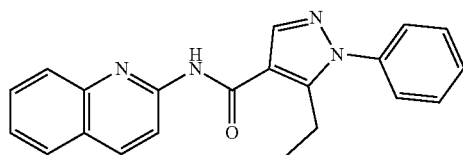
5-ethyl-1-phenyl-N-(quinolin-2-yl)-1H-pyrazole-4-carboxamide (157)
