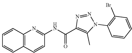
1-(2-Bromophenyl)-5-methyl-N-(quinolin-2-yl)-1H-1,2,3-triazole-4-carboxamide (21)
