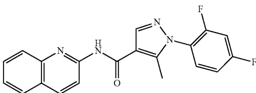
1-(2,4-difluorophenyl)-5-methyl-N-(quinolin-2-yl)-1H-pyrazole-4-carboxamide (140)
