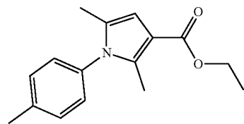
Ethyl 2,5-dimethyl-1-(p-tolyl)-1H-pyrrole-3-carboxylate (12)
