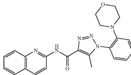
5-Methyl-1-(2-morpholinophenyl)-N-(quinolin-2-yl)-1H-1,2,3-triazole-4-carboxamide (28)
