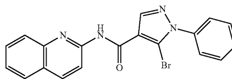
5-bromo-1-phenyl-N-(quinolin-2-yl)-1H-pyrazole-4-carboxamide (160)
