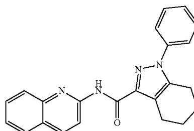
1-phenyl-N-(quinolin-2-yl)-4,5,6,7-tetrahydro-1H-indazole-3-carboxamide (153)
