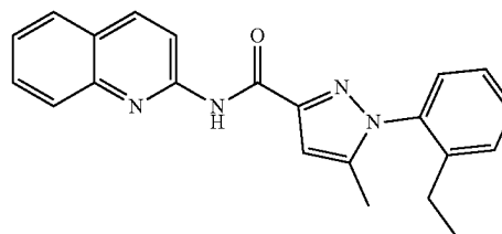
1-(2-ethylphenyl)-5-methyl-N-(quinolin-2-yl)-1H-pyrazole-3-carboxamide (151)
