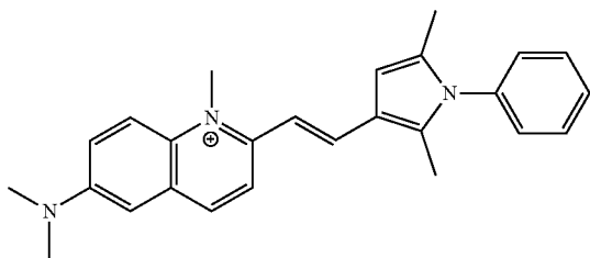
Scheme 1: Pyrvinium Structure
