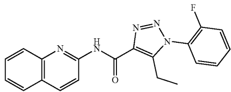
5-Ethyl-1-(2-fluorophenyl)-N-(quinolin-2-yl)-1H-1,2,3-triazole-4-carboxamide (45)
