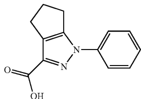
1-phenyl-1,4,5,6-tetrahydrocyclopenta[c]pyrazole-3-carboxylic acid
