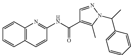
5-methyl-1-(1-phenylethyl)-N-(quinolin-2-yl)-1H-pyrazole-4-carboxamide (143)
