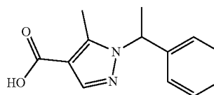
5-methyl-1-(1-phenylethyl)-1H-pyrazole-4-carboxylic acid
