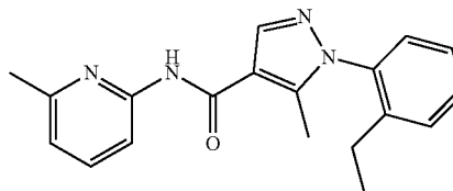
1-(2-ethylphenyl)-5-methyl-N-(6-methylpyridin-2-yl)-1H-pyrazole-4-carboxamide (165)
