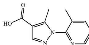
5-Methyl-1-(3-methylpyridin-2-yl)-1H-pyrazole-4-carboxylic acid
