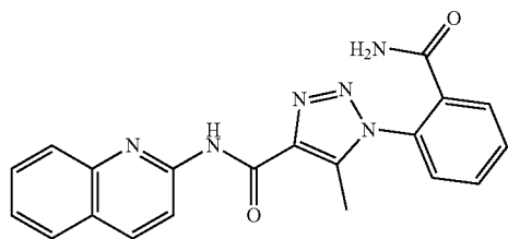
1-(2-Carbamoylphenyl)-5-methyl-N-(quinolin-2-yl)-1H-1,2,3-triazole-4-carboxamide (40)
