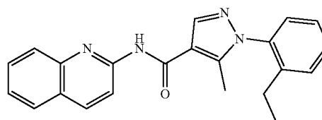
1-(2-Ethylphenyl)-5-methyl-N-(quinolin-2-yl)-1H-pyrazole-4-carboxamide (136)
