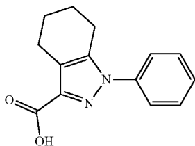
1-phenyl-4,5,6,7-tetrahydro-1H-indazole-3-carboxylic acid
