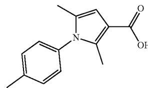
2,5-Dimethyl-1-(p-tolyl)-1H-pyrrole-3-carboxylic acid (13)
