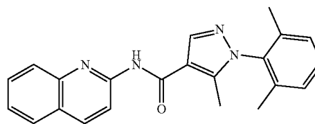
1-(2,6-dimethylphenyl)-5-methyl-N-(quinolin-2-yl)-1H-pyrazole-4-carboxamide (137)
