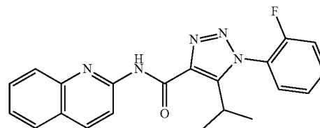
1-(2-Fluorophenyl)-5-isopropyl-N-(quinolin-2-yl)-1H-1,2,3-triazole-4-carboxamide (46)
