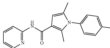
2,5-dimethyl-N-(pyridin-2-yl)-1-(p-tolyl)-1H-pyrrole-3-carboxamide (14)
