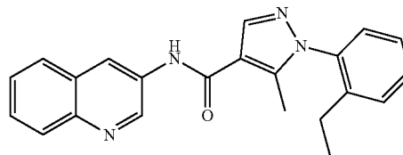
1-(2-ethylphenyl)-5-methyl-N-(quinolin-3-yl)-1H-pyrazole-4-carboxamide (164)
