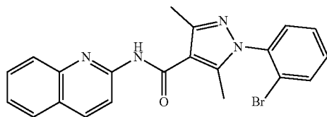
1-(2-bromophenyl)-3,5-dimethyl-N-(quinolin-2-yl)-1H-pyrazole-4-carboxamide (156)
