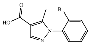
1-(2-Bromophenyl)-5-methyl-1H-pyrazole-4-carboxylic acid
