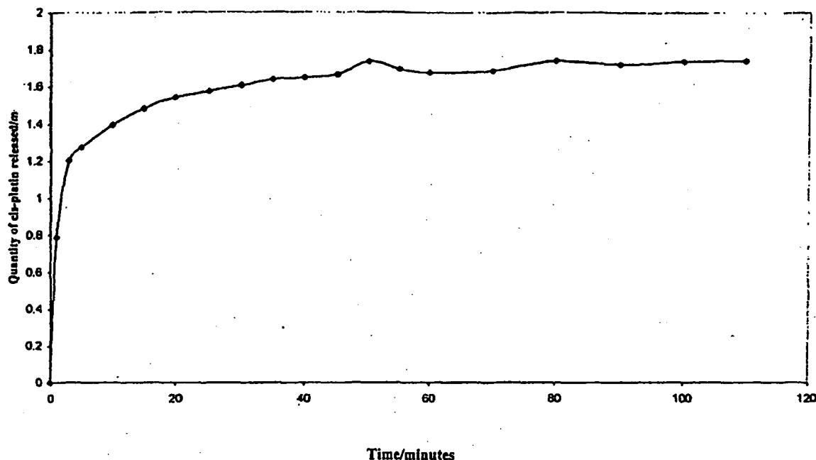
Leaching of [\text{Fe}(\text{phen})_3][\text{ClO}_4]_2 from HA loaded with PLG
