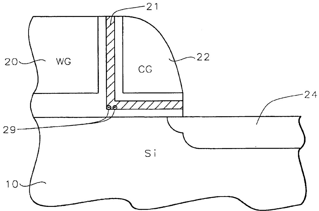
FIG. 4 Prior Art
