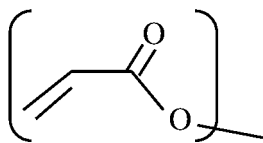
Acrylate Group
