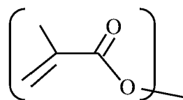
Methacrylate Group
