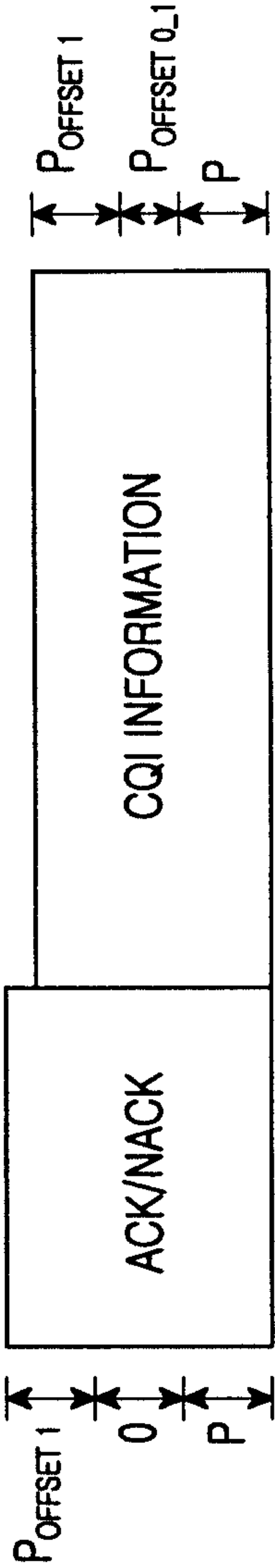
FIG. 5D HS-DPCCH
