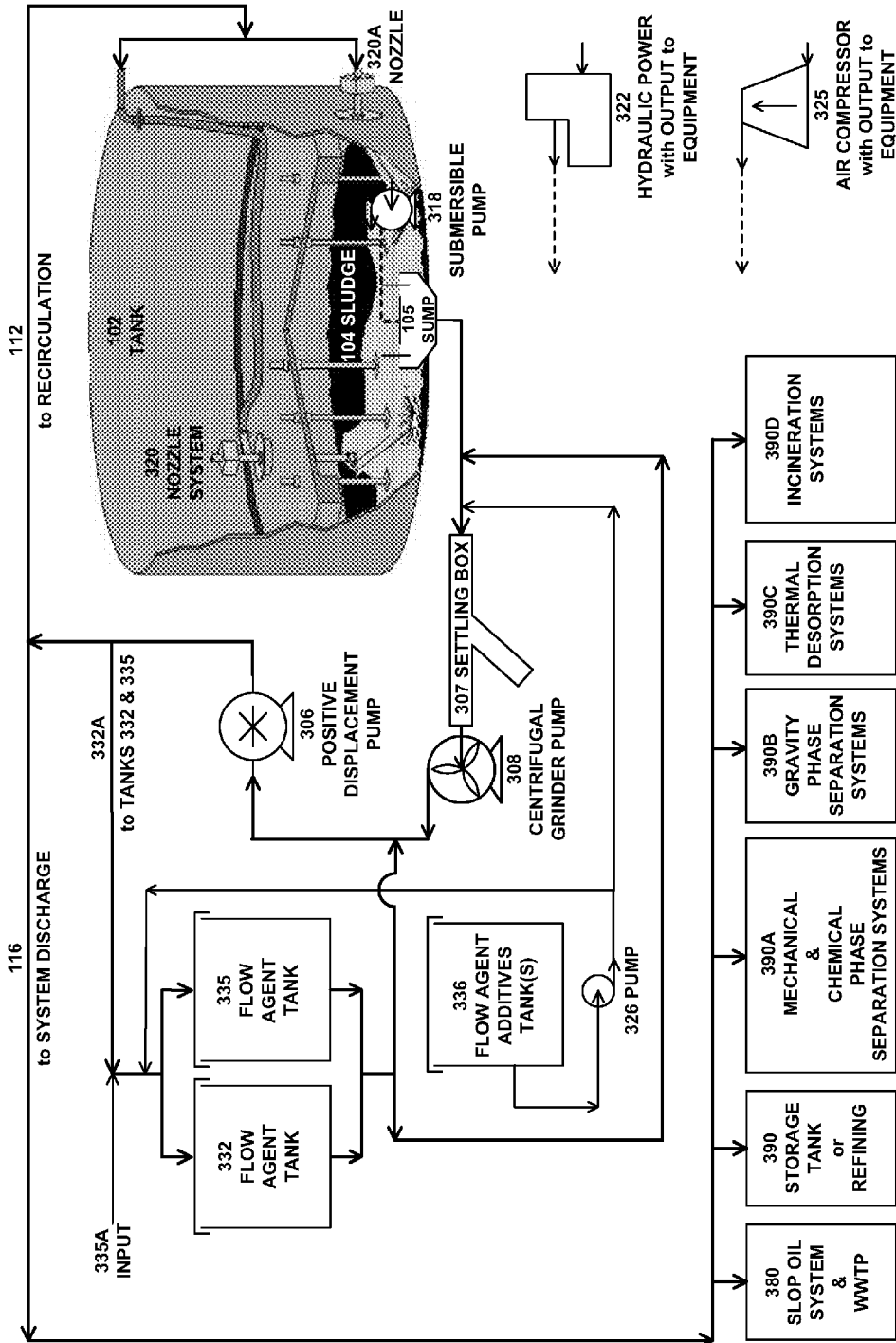
Figure 3 300 HYDROCARBON STORAGE TANK SLUDGE REMOVAL AND CLEANING SYSTEM
