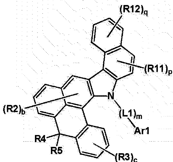
[Chemical Formula 8]
