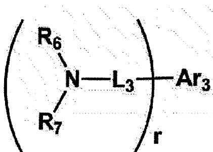
[Chemical Formula 14]
