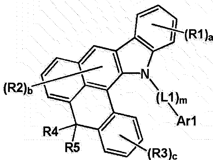
[Chemical Formula 2-2]
