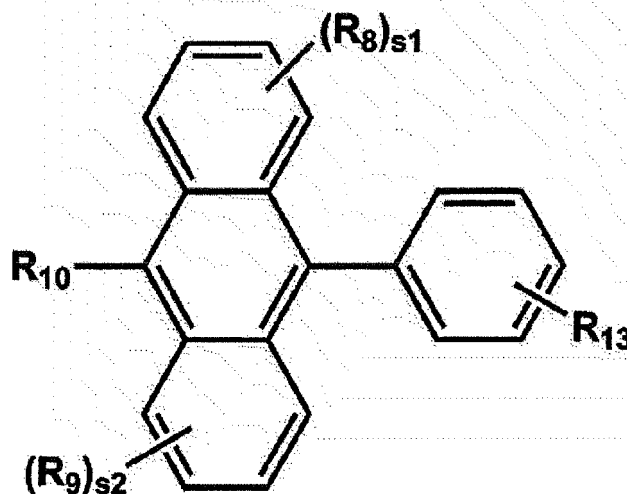
[Chemical Formula 15]
