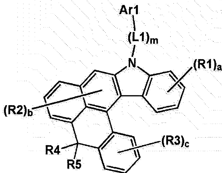
[Chemical Formula 2-2]
