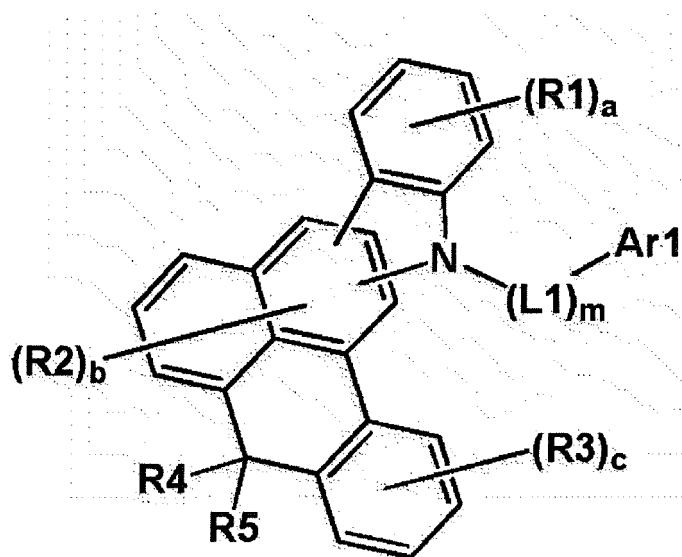
[Chemical Formula 1]
