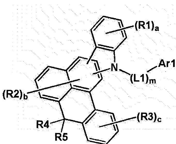
[Chemical Formula 1]
