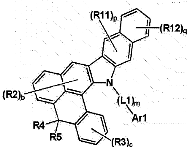
[Chemical Formula 8]
