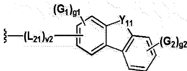
[Chemical Formula 10]
