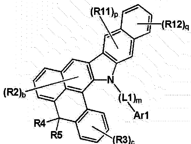
[Chemical Formula 8]
