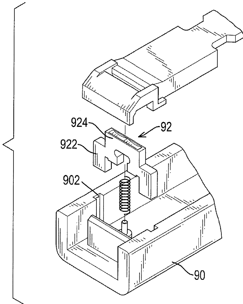
FIG.5 PRIOR ART
