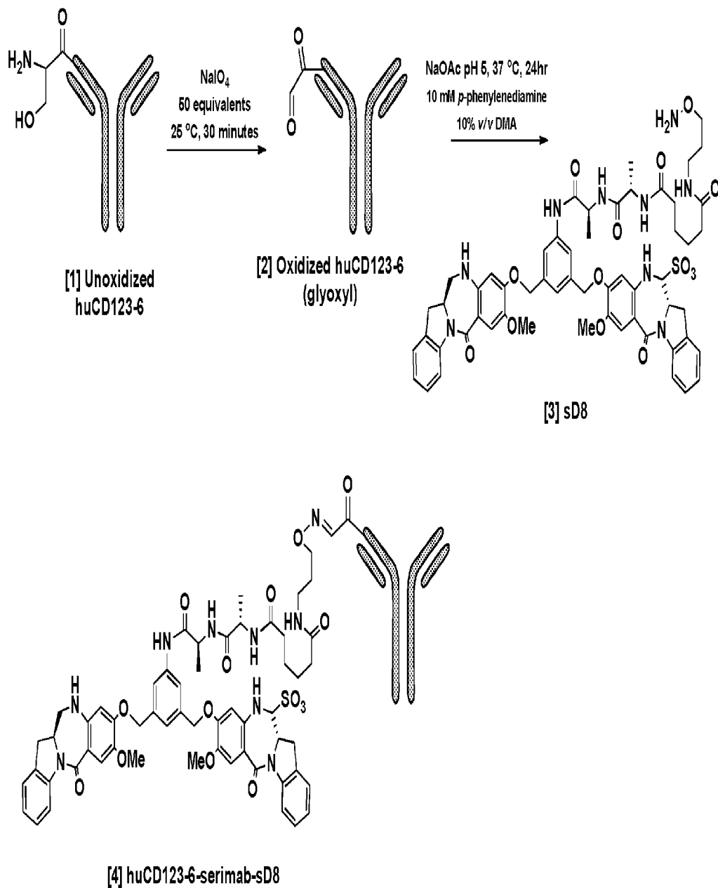
Scheme 2
