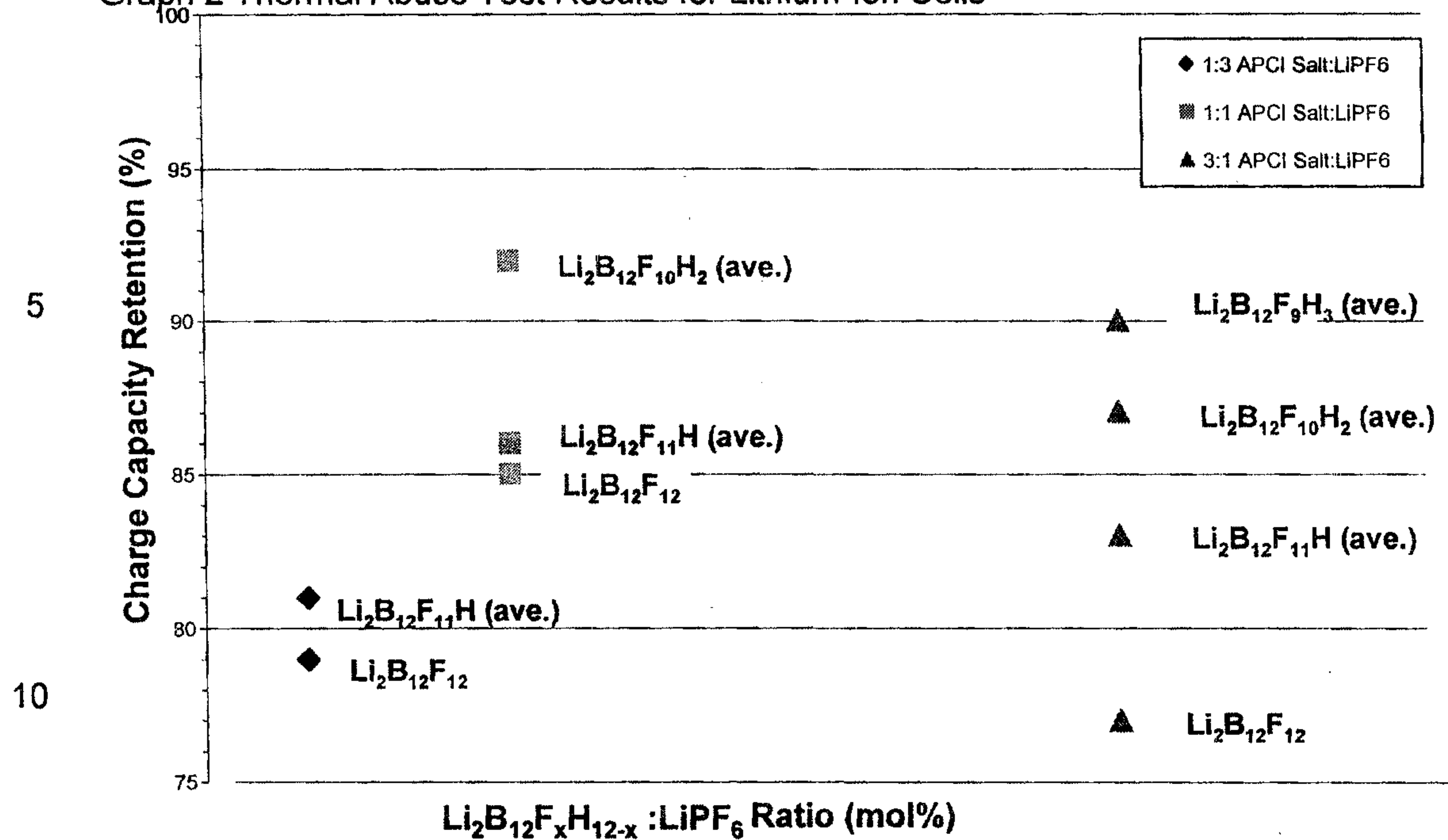
Graph 2 Thermal Abuse Test Results for Lithium-Ion Cells
