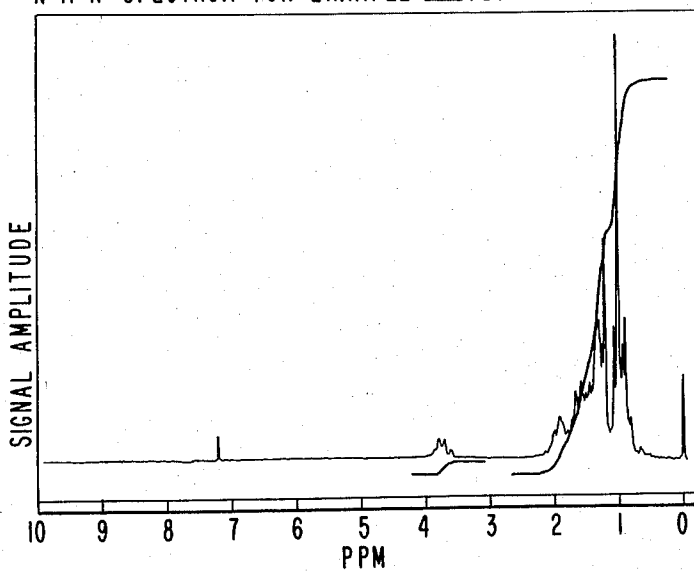
N M R SPECTRUM FOR EXAMPLE VII(B).
