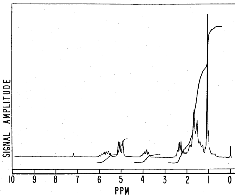
NMR SPECTRUM FOR EXAMPLE V(B).
