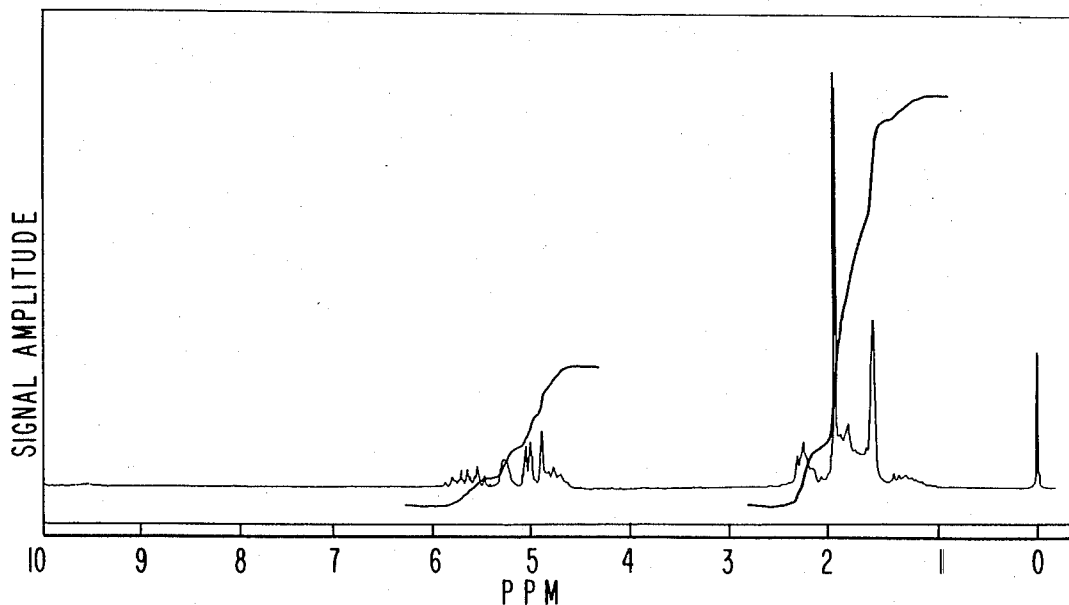
N M R SPECTRUM FOR EXAMPLE XXXIV.
