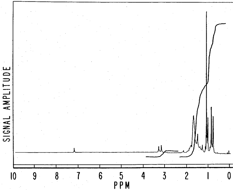
NMR SPECTRUM FOR EXAMPLE VIII
