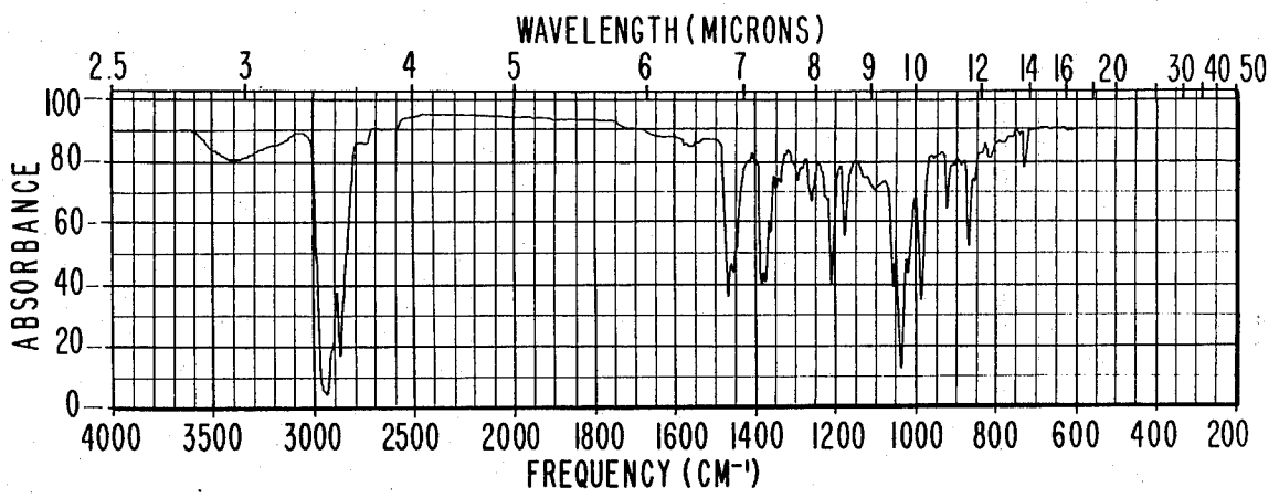
IR SPECTRUM FOR EXAMPLE VIII.
