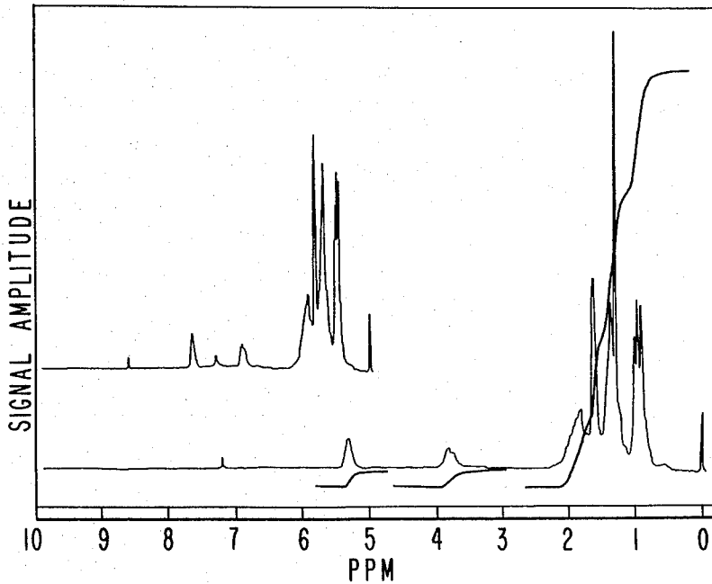
N M R SPECTRUM FOR EXAMPLE VII(A).
