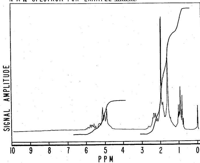
NMR SPECTRUM FOR EXAMPLE XXXIII
