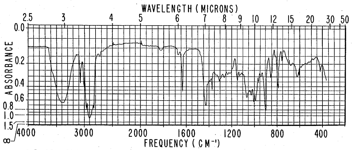
I R SPECTRUM FOR EXAMPLE V (A).
