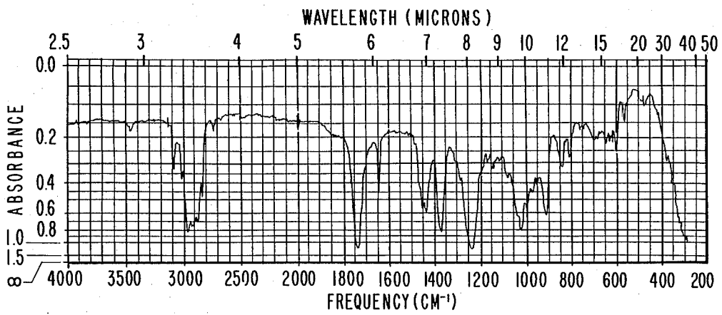
IR SPECTRUM FOR EXAMPLE XXXIII .
