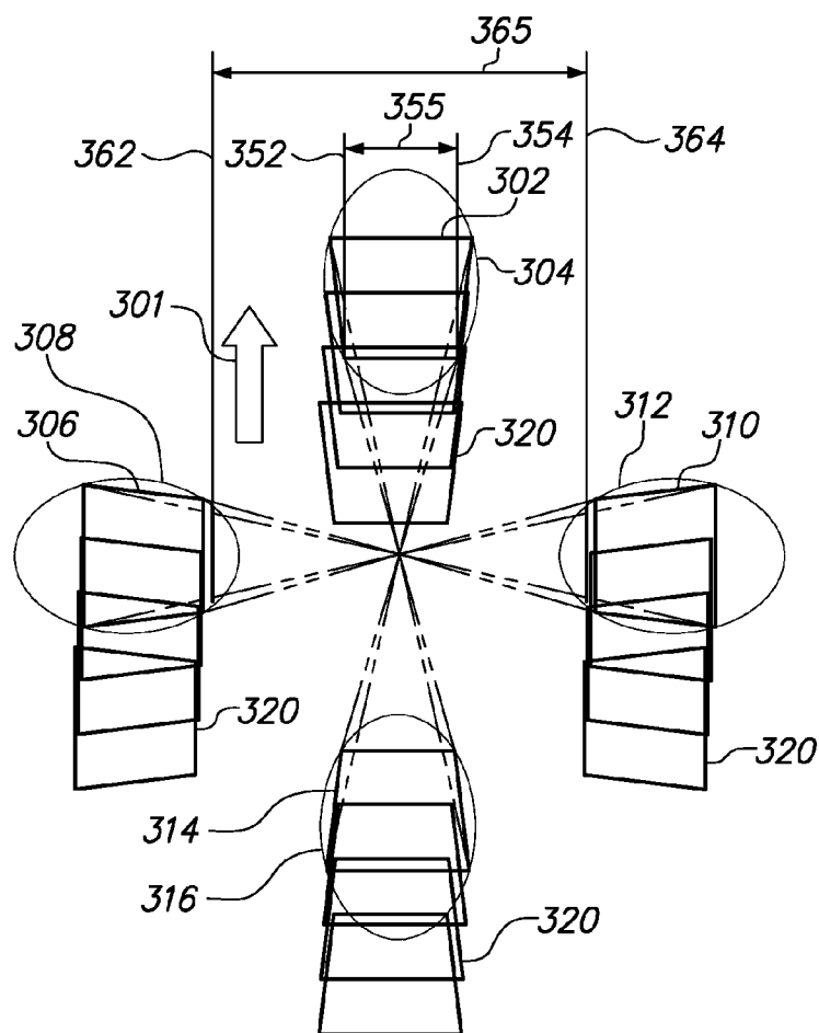
FIG. 3 (Prior Art)
