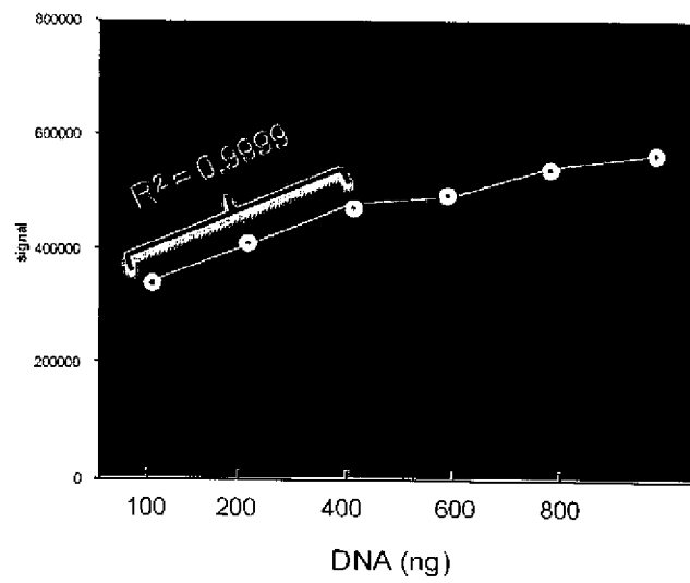
5-METHYLCYTOSINE IR
