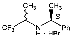
[Chem. 11]
