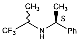
[Chem. 10]
