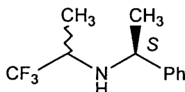
[Chem. 8]
