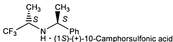
[Chem. 15]
