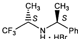
[Chem. 12]
