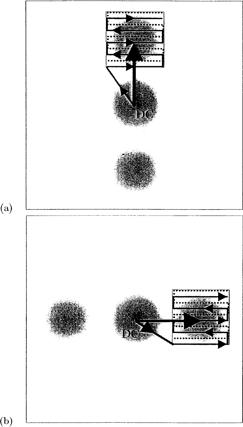
Figure 1: Acquisition of 1-D, 1-1 SPAMM spectral peaks for (a) horizontal tags and (b) vertical tags.
