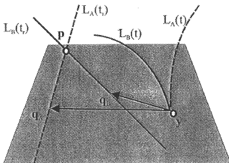
Figure 12: 3-D CHARP tracks image point y back to its material reference point p , which may be out of the image plane.
