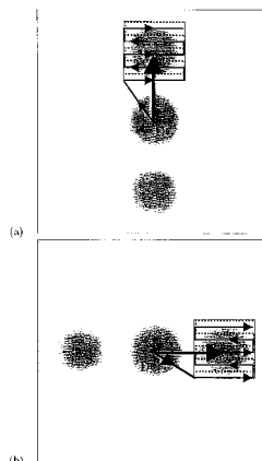
Acquisition of 3-D, 3-1 SPAMM spectral peaks for (a) horizontal tags and (b) vertical tags.
