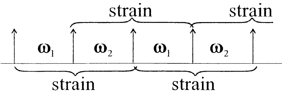
Figure 3: Successive calculation of strain with alternating tag orientations.
