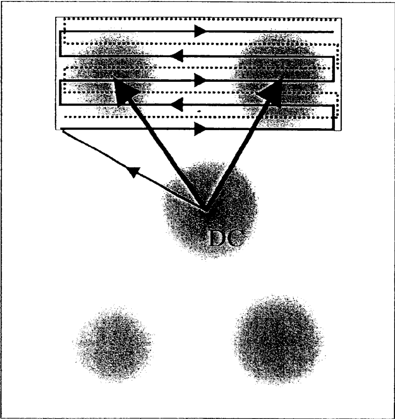
Figure 5: Simultaneous acquisition of two (2) linearly independent spectral peaks using multi-shot EPI.
