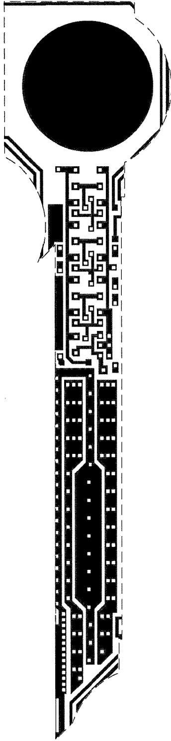
Metal 1 mask
