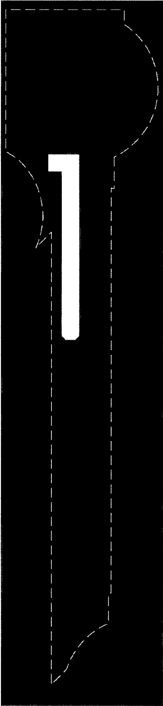
N-Well mask
