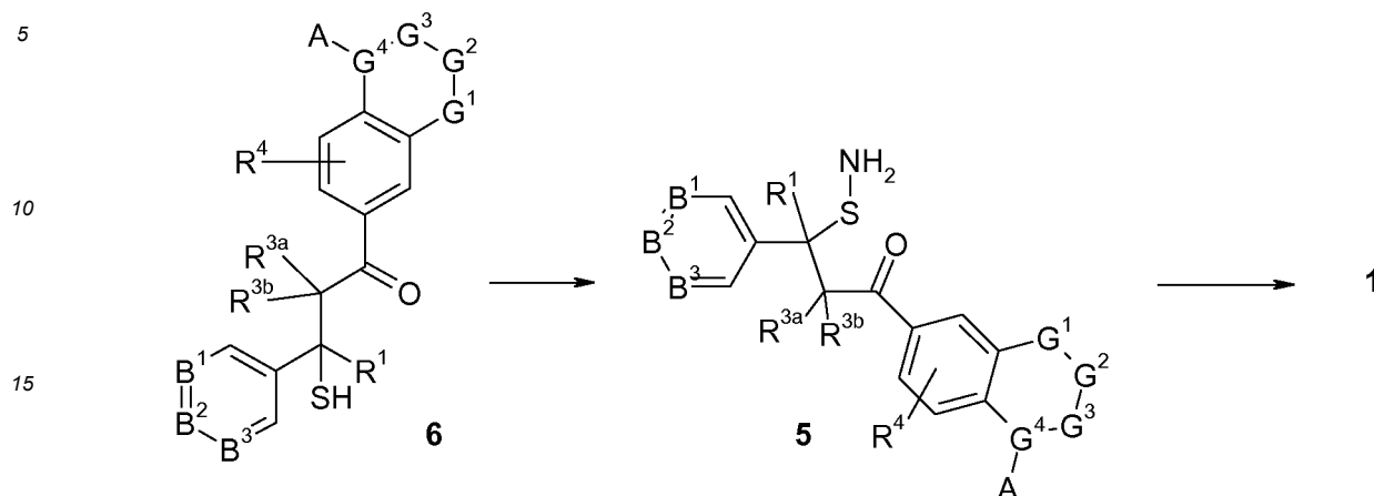
Scheme 3
