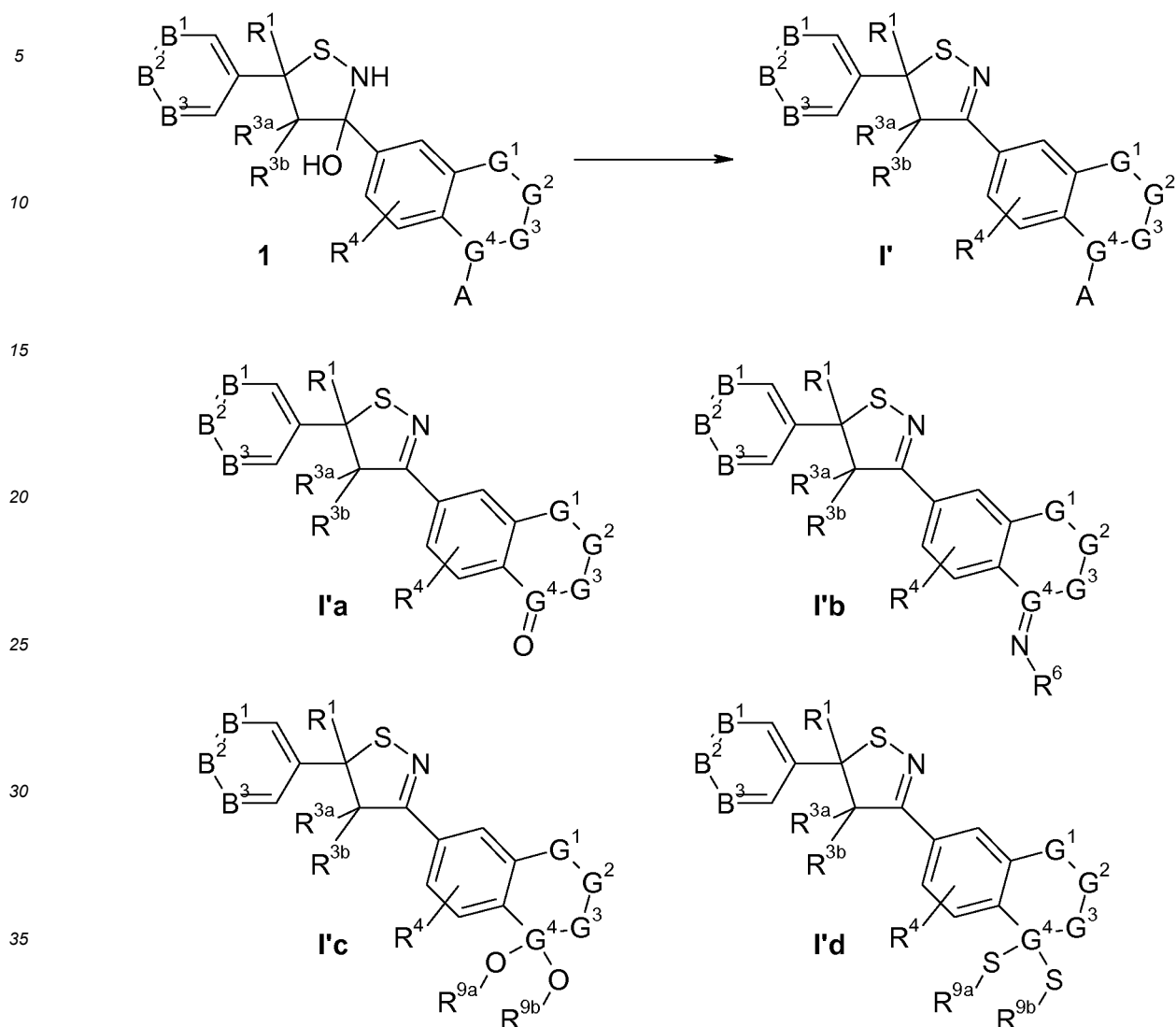
Scheme 1
