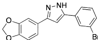
5-(3-Bromophenyl)-3-(3,4-methylenedioxyphenyl)-1H-pyrazole
