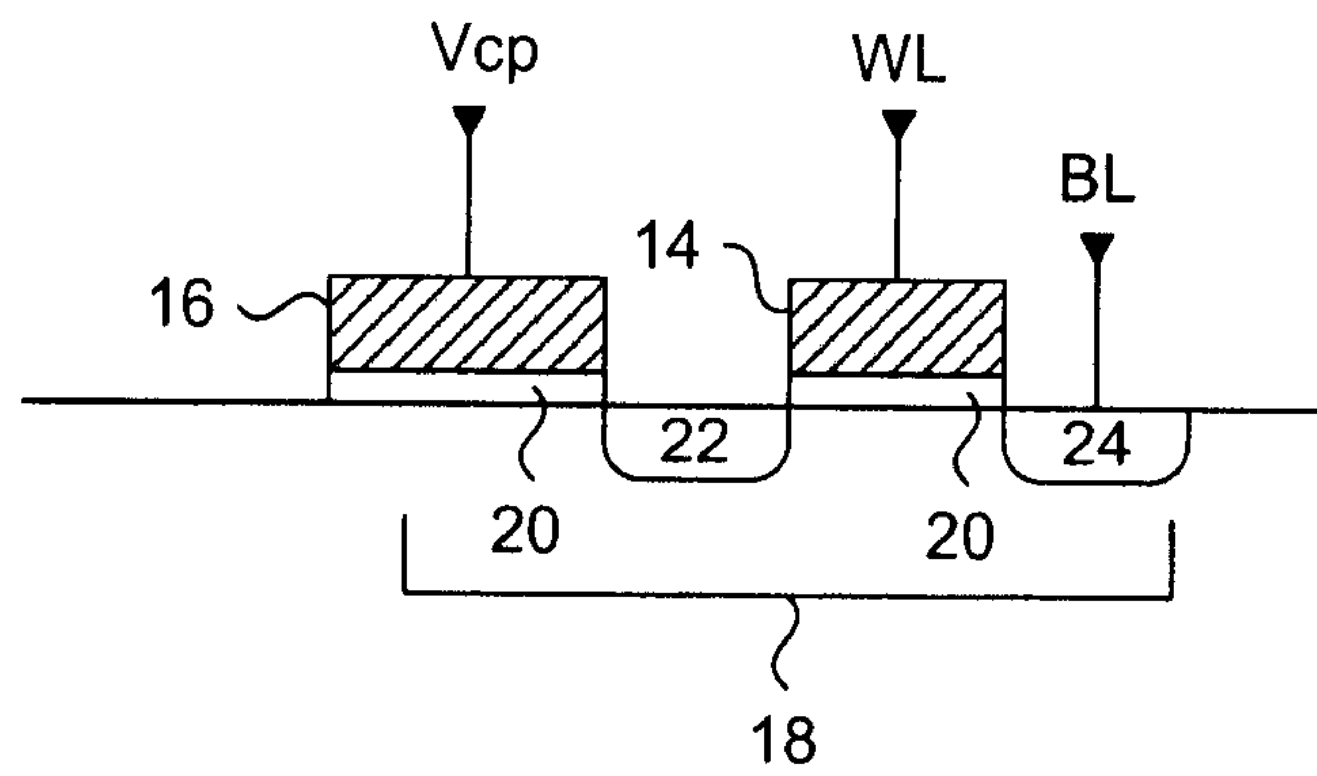
FIG. 3 (Prior Art)
