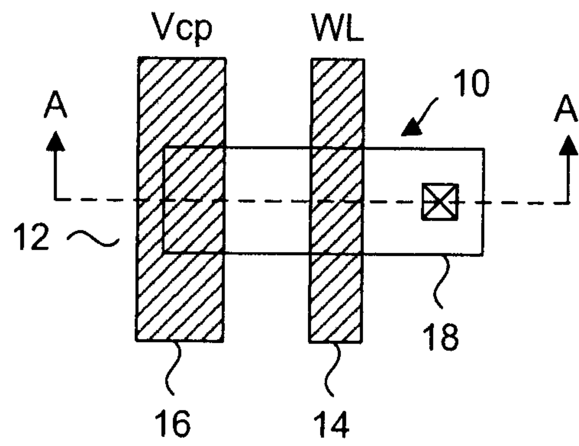
FIG. 2 (Prior Art)
