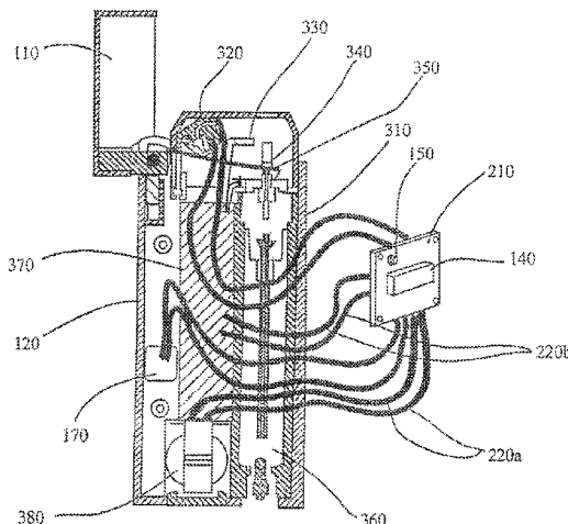
Portable Biometric Lighter Cross-Sectional View
