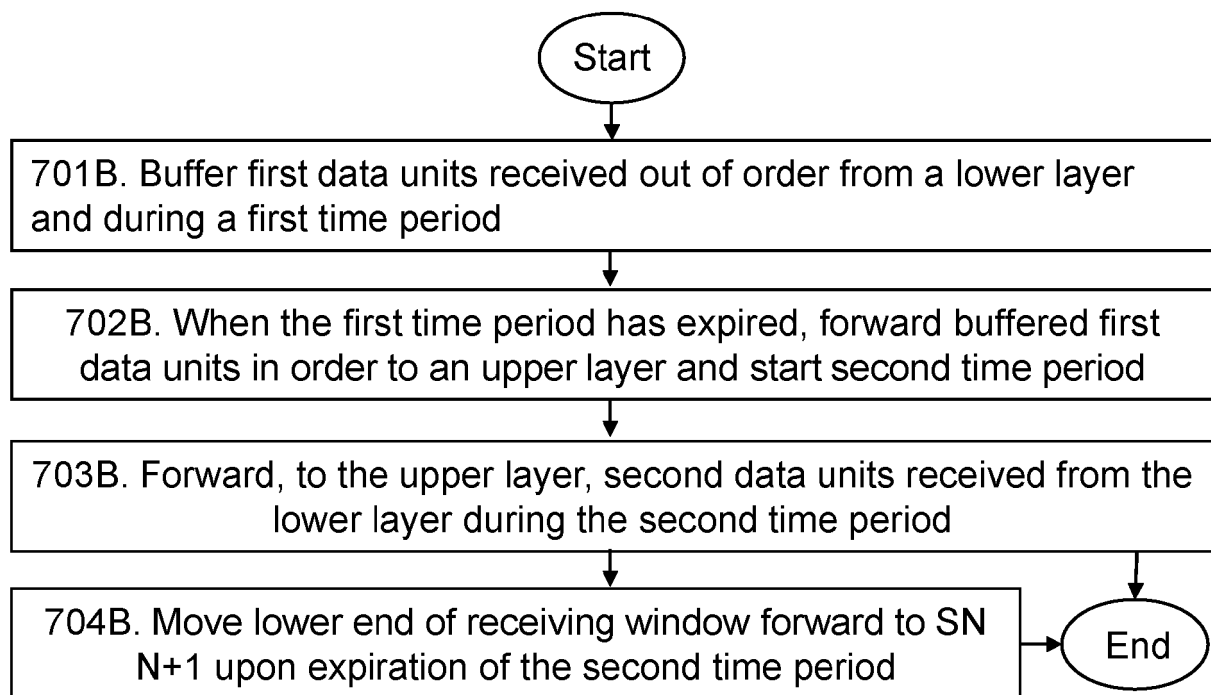
Figure 7B Method performed by network node 606, 608
